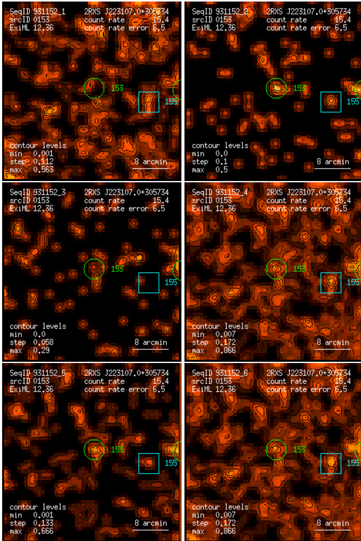
Figure 153: RASS 931152: detection 0153: band rate images, Gaussian filter: (1) PSPC channels 11 – 41, (2) 52 – 90, (3) 91 – 201, (4) 11 – 235, (5) 52 – 201, (6) 11 – 201. Broad band rates in counts/ks. Band rate contour levels in counts/ks/arcmin 2 .
