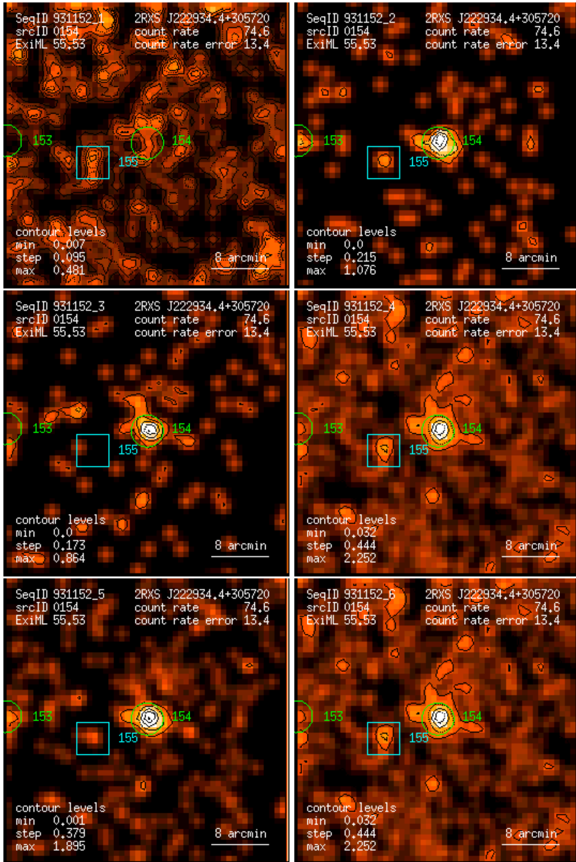
Figure 154: RASS 931152: detection 0154: band rate images, Gaussian filter: (1) PSPC channels 11 – 41, (2) 52 – 90, (3) 91 – 201, (4) 11 – 235, (5) 52 – 201, (6) 11 – 201. Broad band rates in counts/ks. Band rate contour levels in counts/ks/arcmin 2 .
