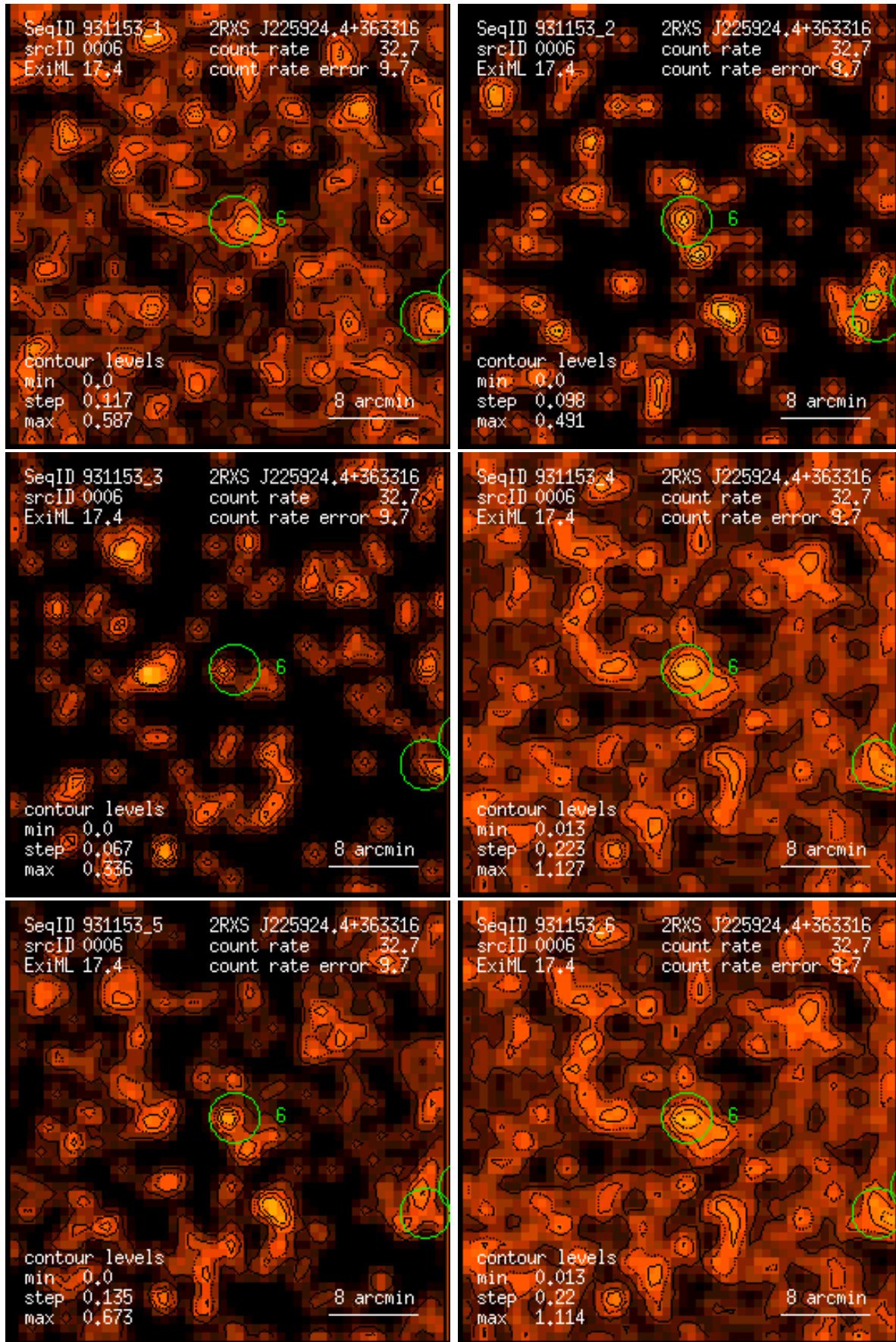
Figure 6: RASS 931153: detection 0006: band rate images, Gaussian filter: (1) PSPC channels 11 – 41, (2) 52 – 90, (3) 91 – 201, (4) 11 – 235, (5) 52 – 201, (6) 11 – 201. Broad band rates in counts/ks. Band rate contour levels in counts/ks/arcmin 2 .
