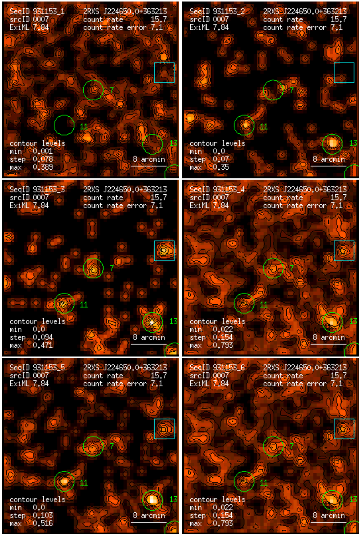
Figure 7: RASS 931153: detection 0007: band rate images, Gaussian filter: (1) PSPC channels 11 – 41, (2) 52 – 90, (3) 91 – 201, (4) 11 – 235, (5) 52 – 201, (6) 11 – 201. Broad band rates in counts/ks. Band rate contour levels in counts/ks/arcmin 2 .
