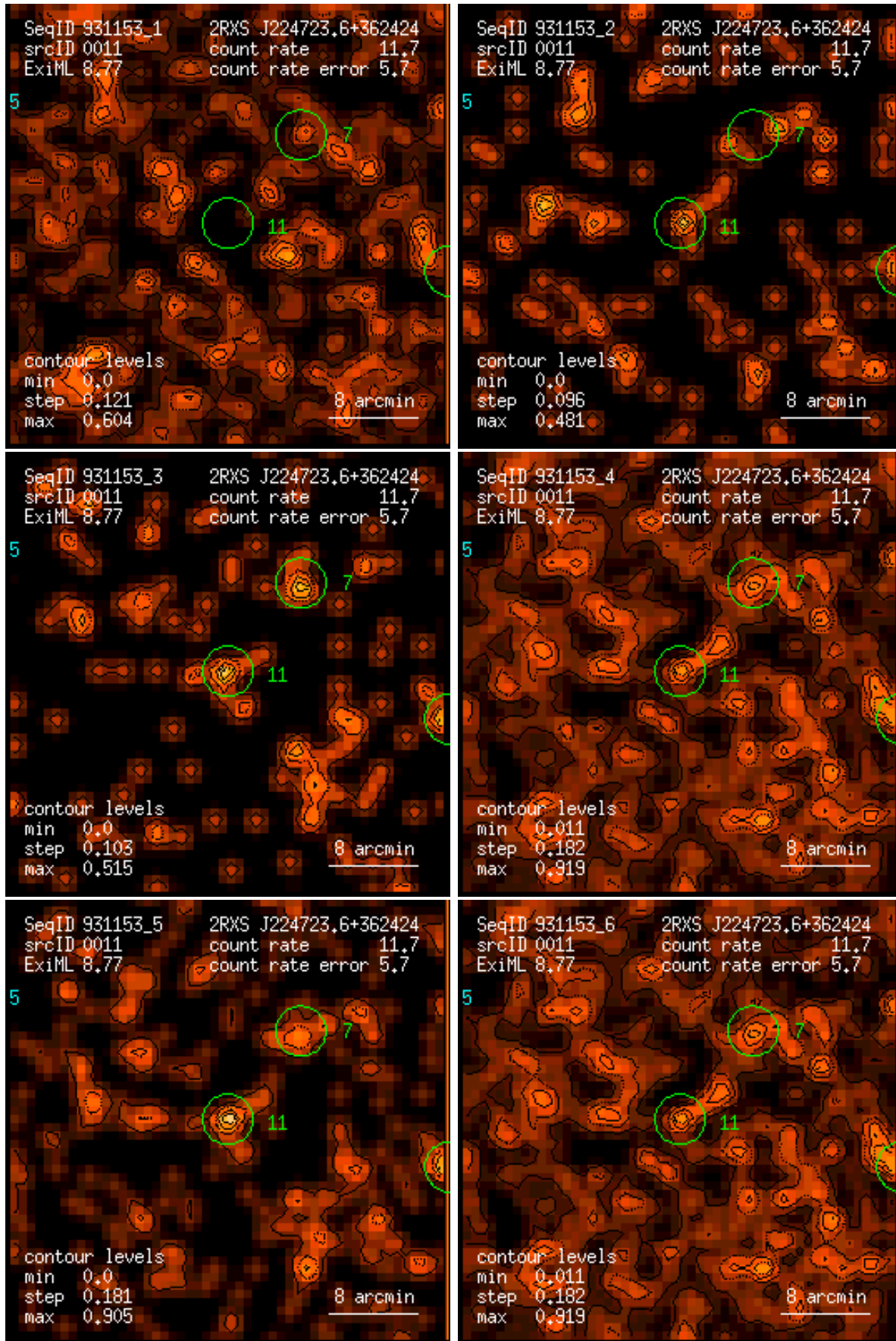
Figure 11: RASS 931153: detection 0011: band rate images, Gaussian filter: (1) PSPC channels 11 – 41, (2) 52 – 90, (3) 91 – 201, (4) 11 – 235, (5) 52 – 201, (6) 11 – 201. Broad band rates in counts/ks. Band rate contour levels in counts/ks/arcmin 2 .
