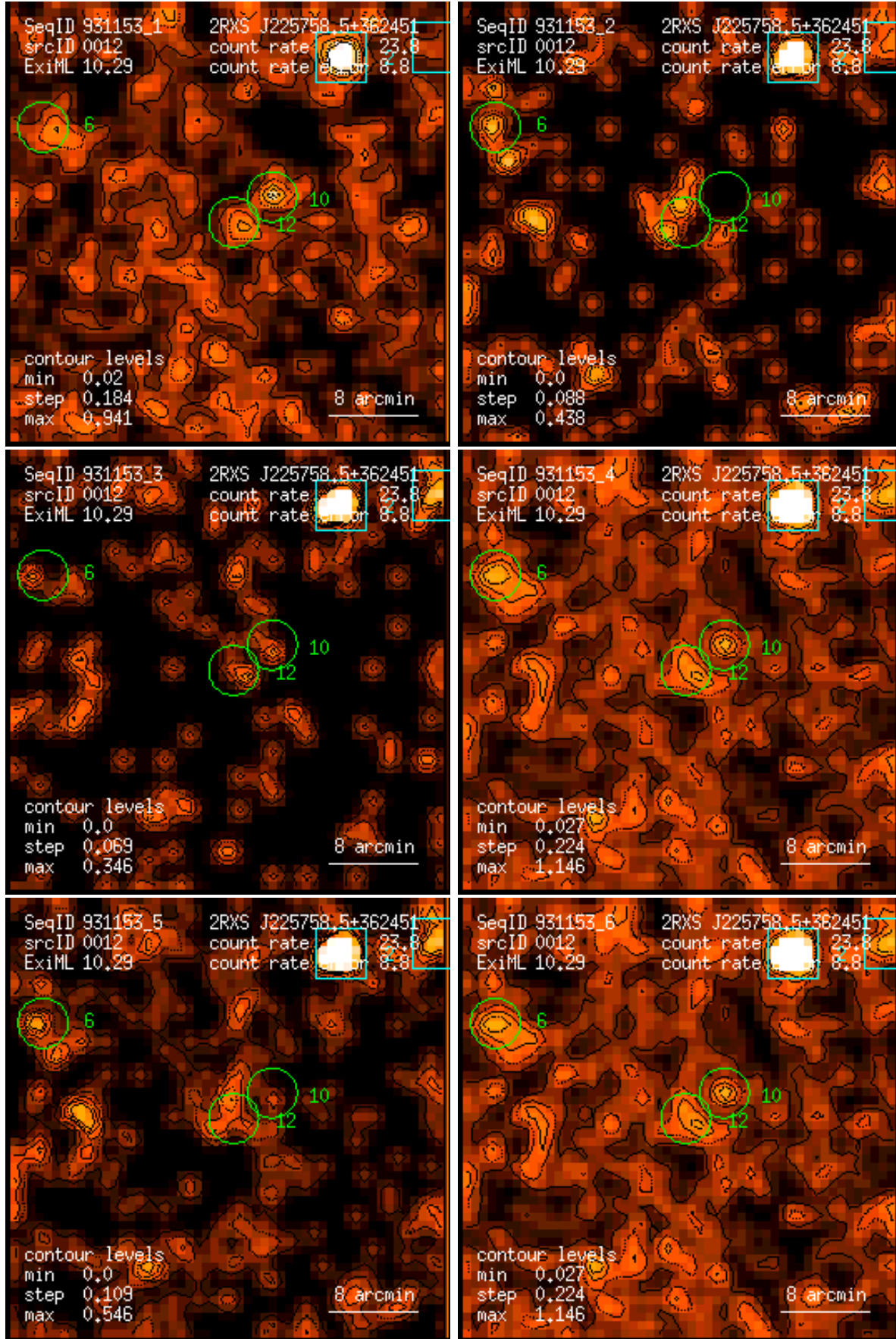
Figure 12: RASS 931153: detection 0012: band rate images, Gaussian filter: (1) PSPC channels 11 – 41, (2) 52 – 90, (3) 91 – 201, (4) 11 – 235, (5) 52 – 201, (6) 11 – 201. Broad band rates in counts/ks. Band rate contour levels in counts/ks/arcmin 2 .
