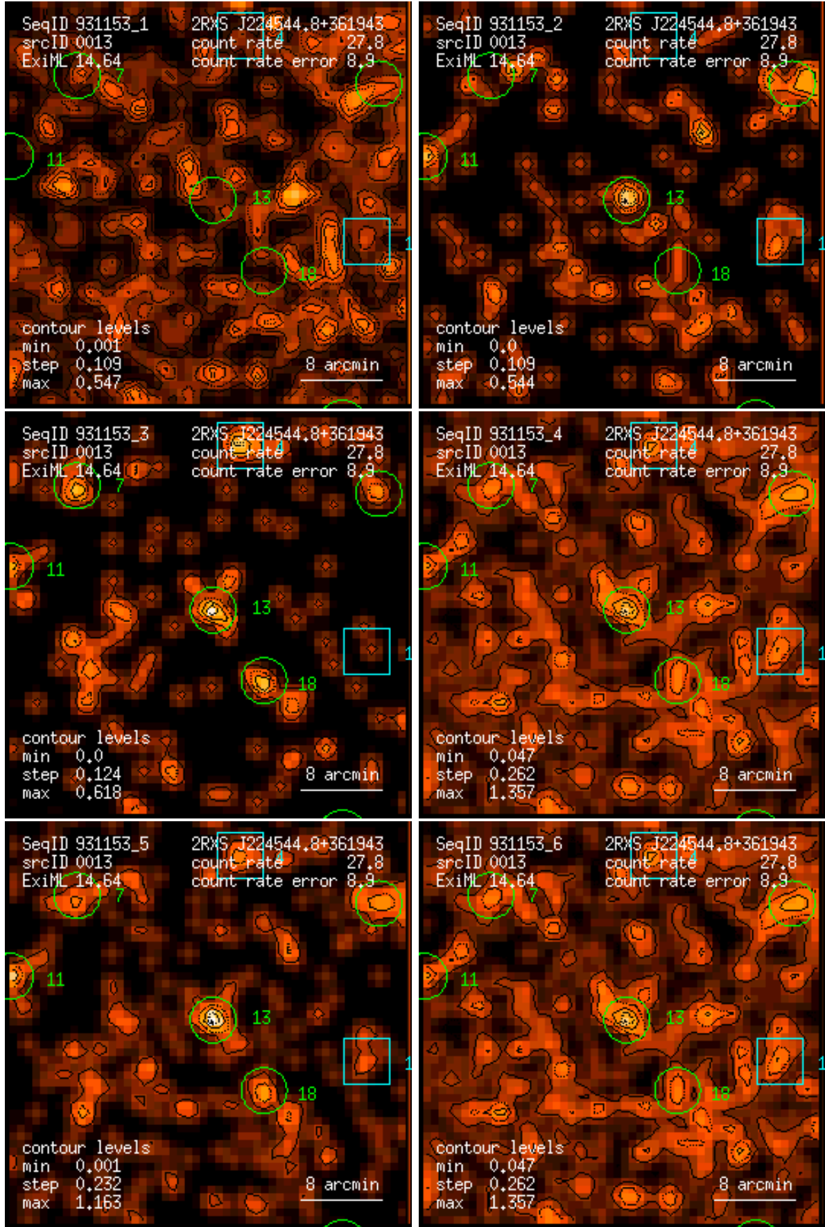
Figure 13: RASS 931153: detection 0013: band rate images, Gaussian filter: (1) PSPC channels 11 – 41, (2) 52 – 90, (3) 91 – 201, (4) 11 – 235, (5) 52 – 201, (6) 11 – 201. Broad band rates in counts/ks. Band rate contour levels in counts/ks/arcmin 2 .
