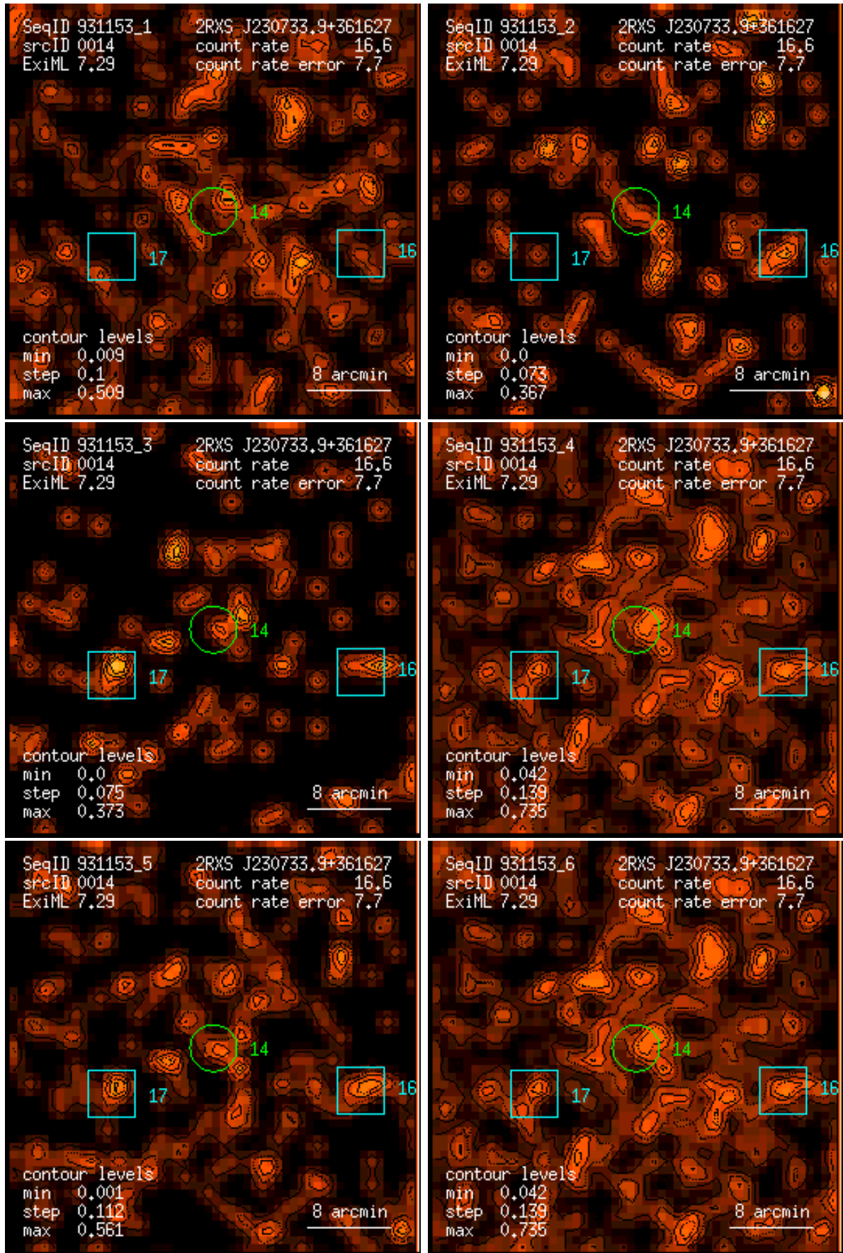
Figure 14: RASS 931153: detection 0014: band rate images, Gaussian filter: (1) PSPC channels 11 – 41, (2) 52 – 90, (3) 91 – 201, (4) 11 – 235, (5) 52 – 201, (6) 11 – 201. Broad band rates in counts/ks. Band rate contour levels in counts/ks/arcmin 2 .
