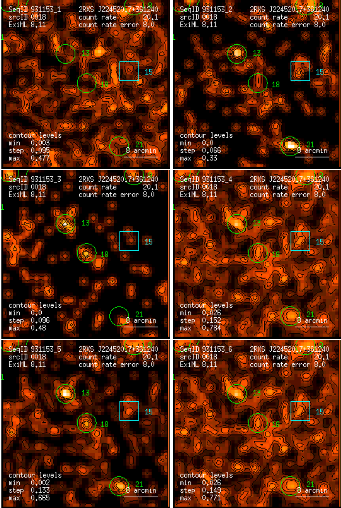
Figure 18: RASS 931153: detection 0018: band rate images, Gaussian filter: (1) PSPC channels 11 – 41, (2) 52 – 90, (3) 91 – 201, (4) 11 – 235, (5) 52 – 201, (6) 11 – 201. Broad band rates in counts/ks. Band rate contour levels in counts/ks/arcmin 2 .
