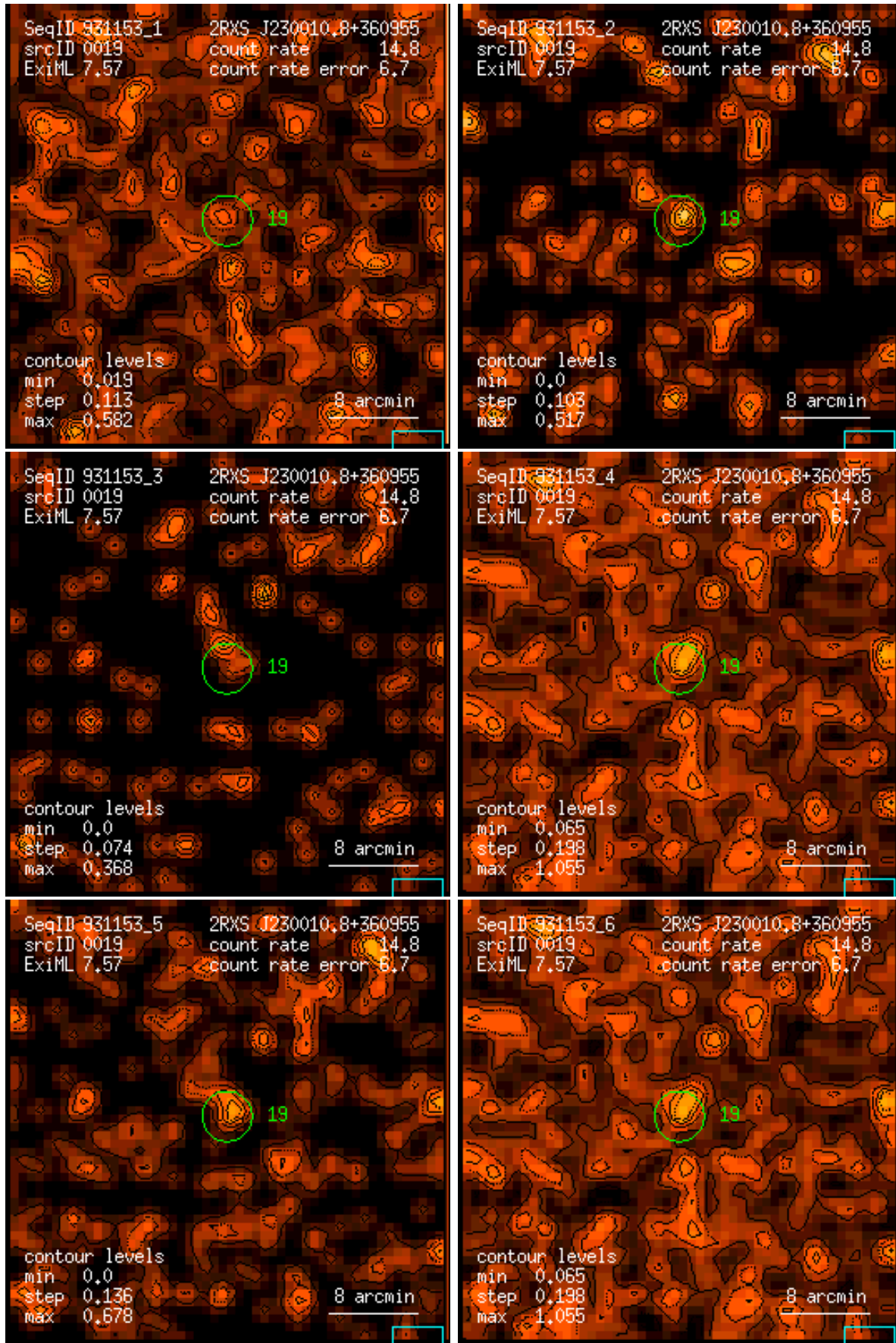
Figure 19: RASS 931153: detection 0019: band rate images, Gaussian filter: (1) PSPC channels 11 – 41, (2) 52 – 90, (3) 91 – 201, (4) 11 – 235, (5) 52 – 201, (6) 11 – 201. Broad band rates in counts/ks. Band rate contour levels in counts/ks/arcmin 2 .
