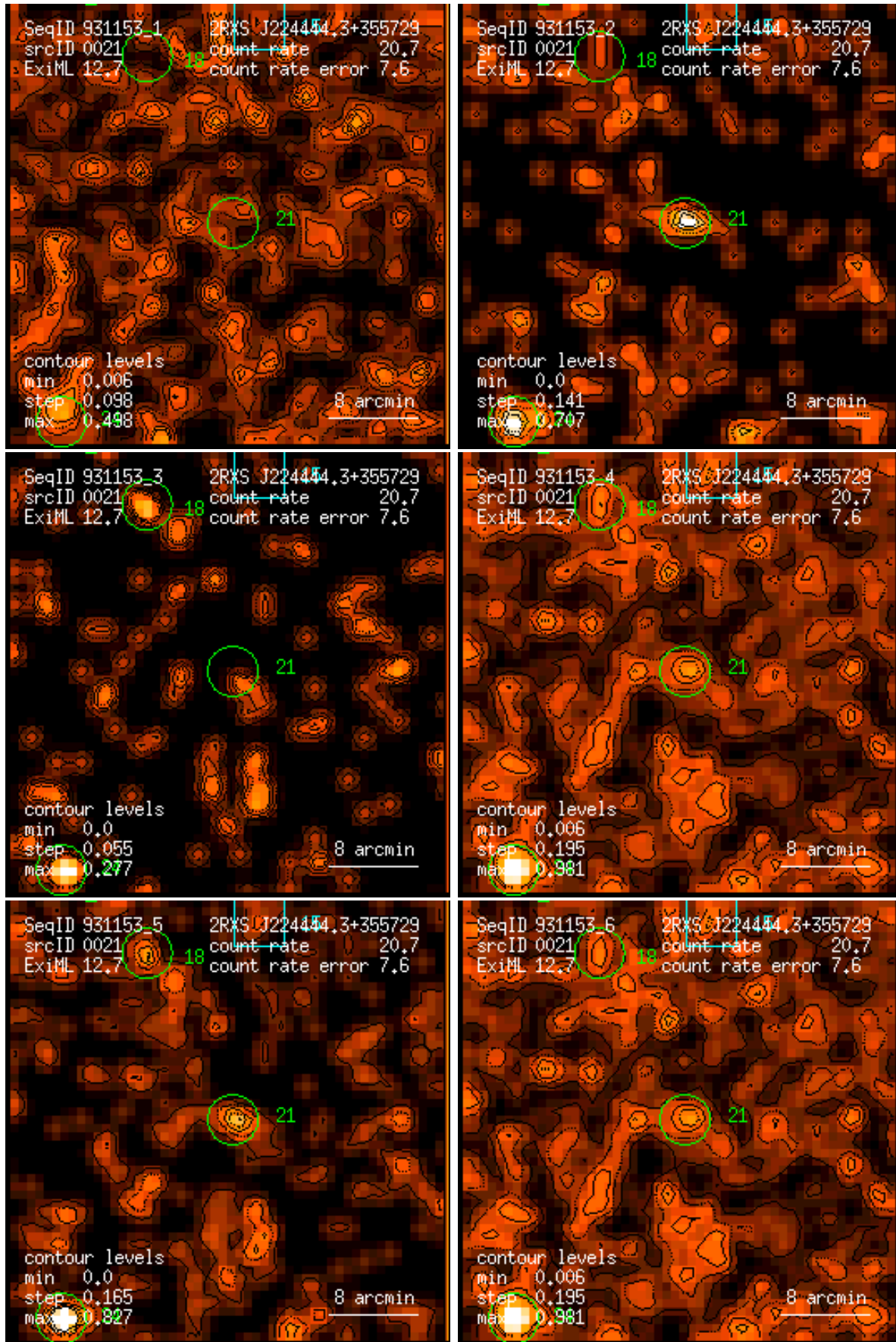
Figure 21: RASS 931153: detection 0021: band rate images, Gaussian filter: (1) PSPC channels 11 – 41, (2) 52 – 90, (3) 91 – 201, (4) 11 – 235, (5) 52 – 201, (6) 11 – 201. Broad band rates in counts/ks. Band rate contour levels in counts/ks/arcmin 2 .
