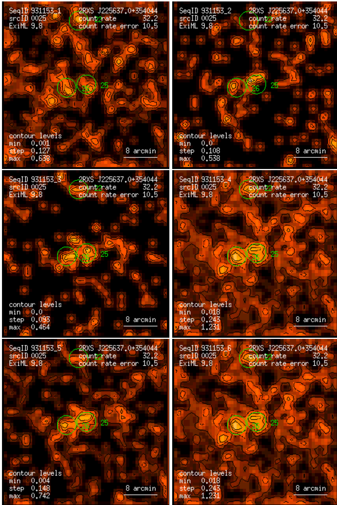
Figure 25: RASS 931153: detection 0025: band rate images, Gaussian filter: (1) PSPC channels 11 – 41, (2) 52 – 90, (3) 91 – 201, (4) 11 – 235, (5) 52 – 201, (6) 11 – 201. Broad band rates in counts/ks. Band rate contour levels in counts/ks/arcmin 2 .
