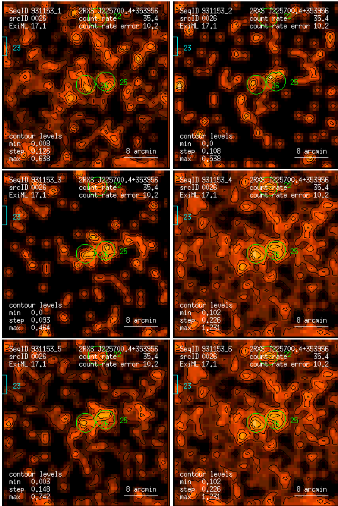
Figure 26: RASS 931153: detection 0026: band rate images, Gaussian filter: (1) PSPC channels 11 – 41, (2) 52 – 90, (3) 91 – 201, (4) 11 – 235, (5) 52 – 201, (6) 11 – 201. Broad band rates in counts/ks. Band rate contour levels in counts/ks/arcmin 2 .
