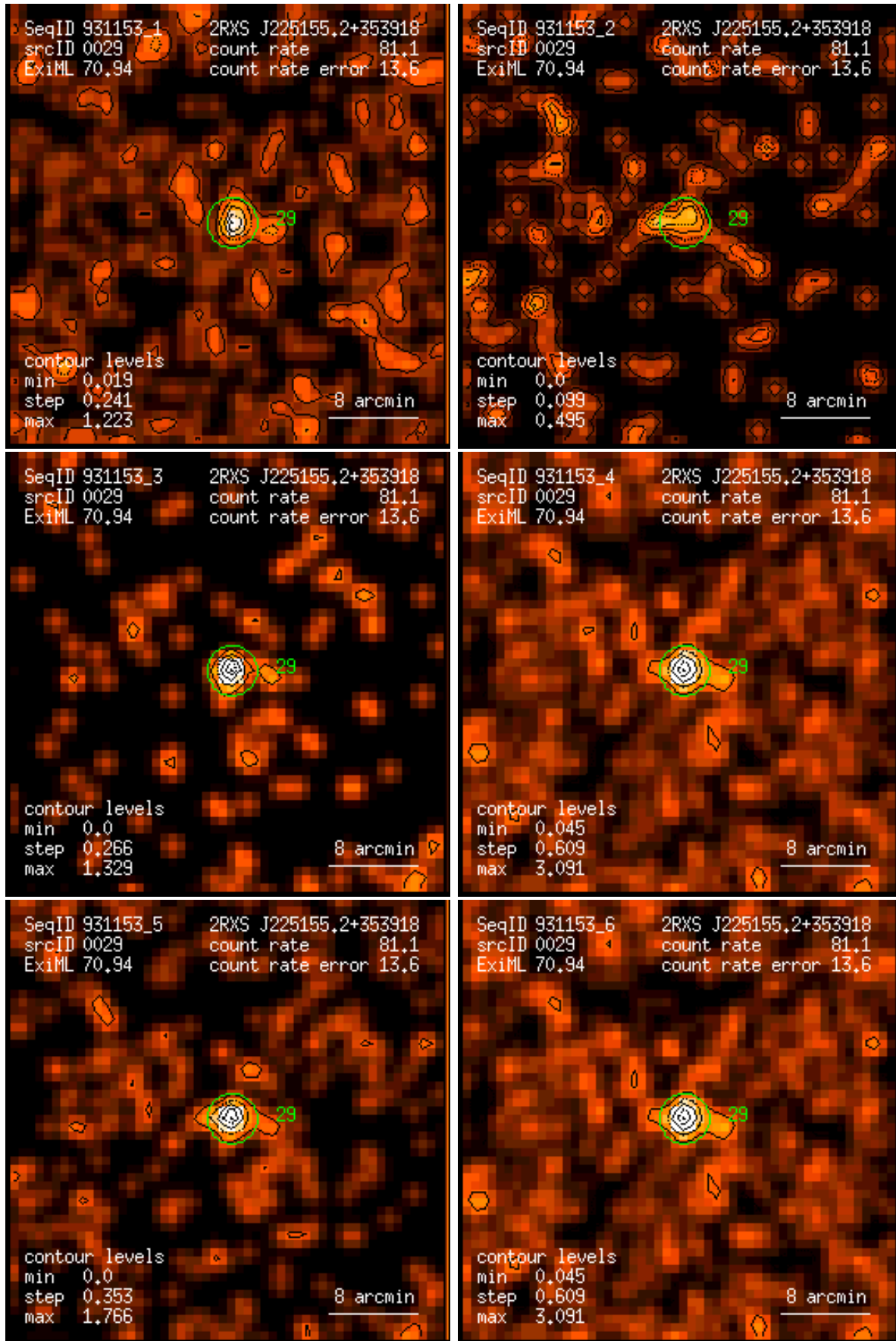
Figure 29: RASS 931153: detection 0029: band rate images, Gaussian filter: (1) PSPC channels 11 – 41, (2) 52 – 90, (3) 91 – 201, (4) 11 – 235, (5) 52 – 201, (6) 11 – 201. Broad band rates in counts/ks. Band rate contour levels in counts/ks/arcmin 2 .
