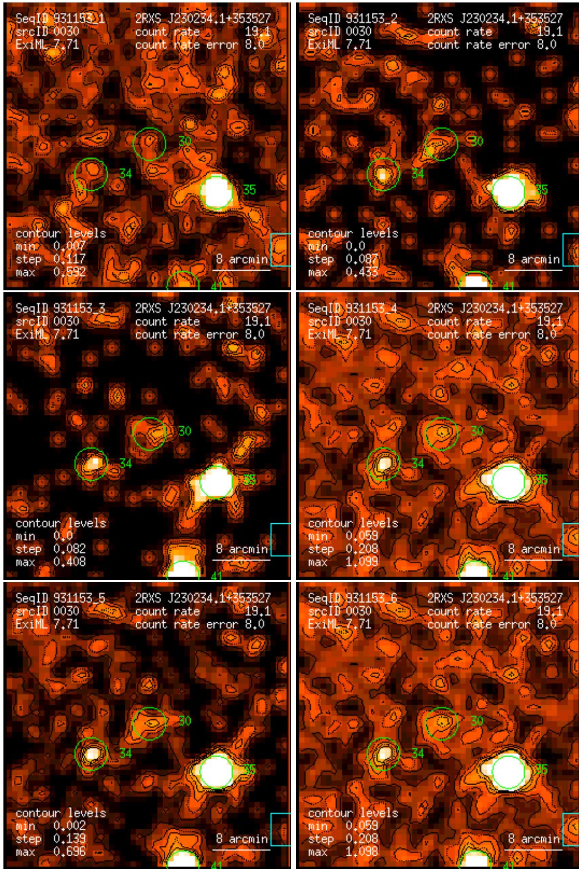
Figure 30: RASS 931153: detection 0030: band rate images, Gaussian filter: (1) PSPC channels 11 – 41, (2) 52 – 90, (3) 91 – 201, (4) 11 – 235, (5) 52 – 201, (6) 11 – 201. Broad band rates in counts/ks. Band rate contour levels in counts/ks/arcmin 2 .
