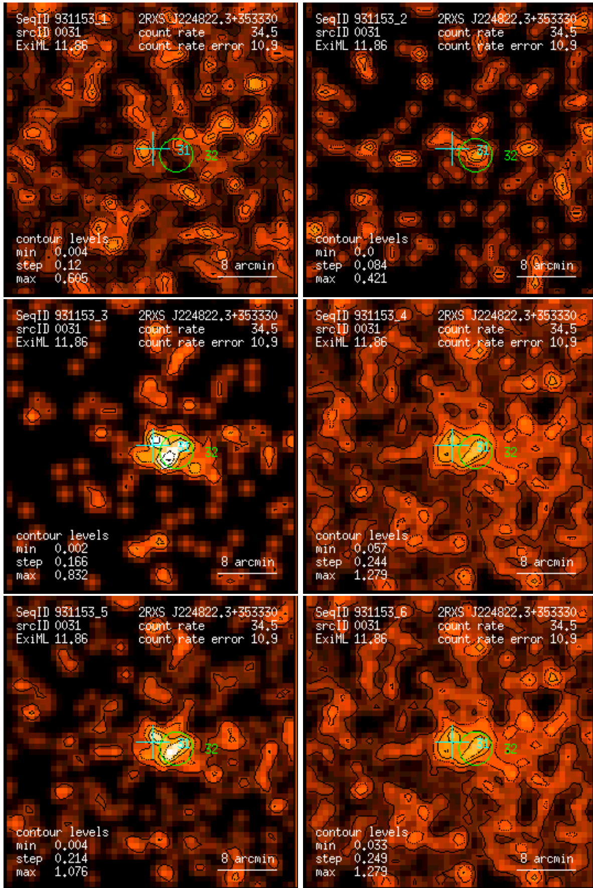
Figure 31: RASS 931153: detection 0031: band rate images, Gaussian filter: (1) PSPC channels 11 – 41, (2) 52 – 90, (3) 91 – 201, (4) 11 – 235, (5) 52 – 201, (6) 11 – 201. Broad band rates in counts/ks. Band rate contour levels in counts/ks/arcmin 2 .
