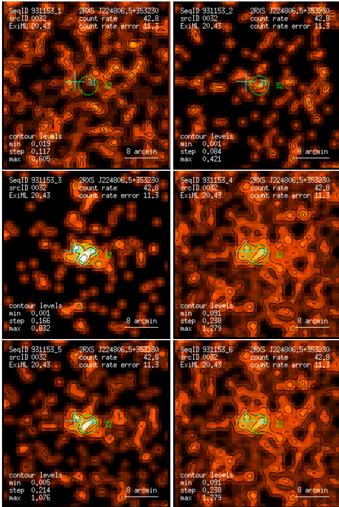
Figure 32: RASS 931153: detection 0032: band rate images, Gaussian filter: (1) PSPC channels 11 – 41, (2) 52 – 90, (3) 91 – 201, (4) 11 – 235, (5) 52 – 201, (6) 11 – 201. Broad band rates in counts/ks. Band rate contour levels in counts/ks/arcmin 2 .
