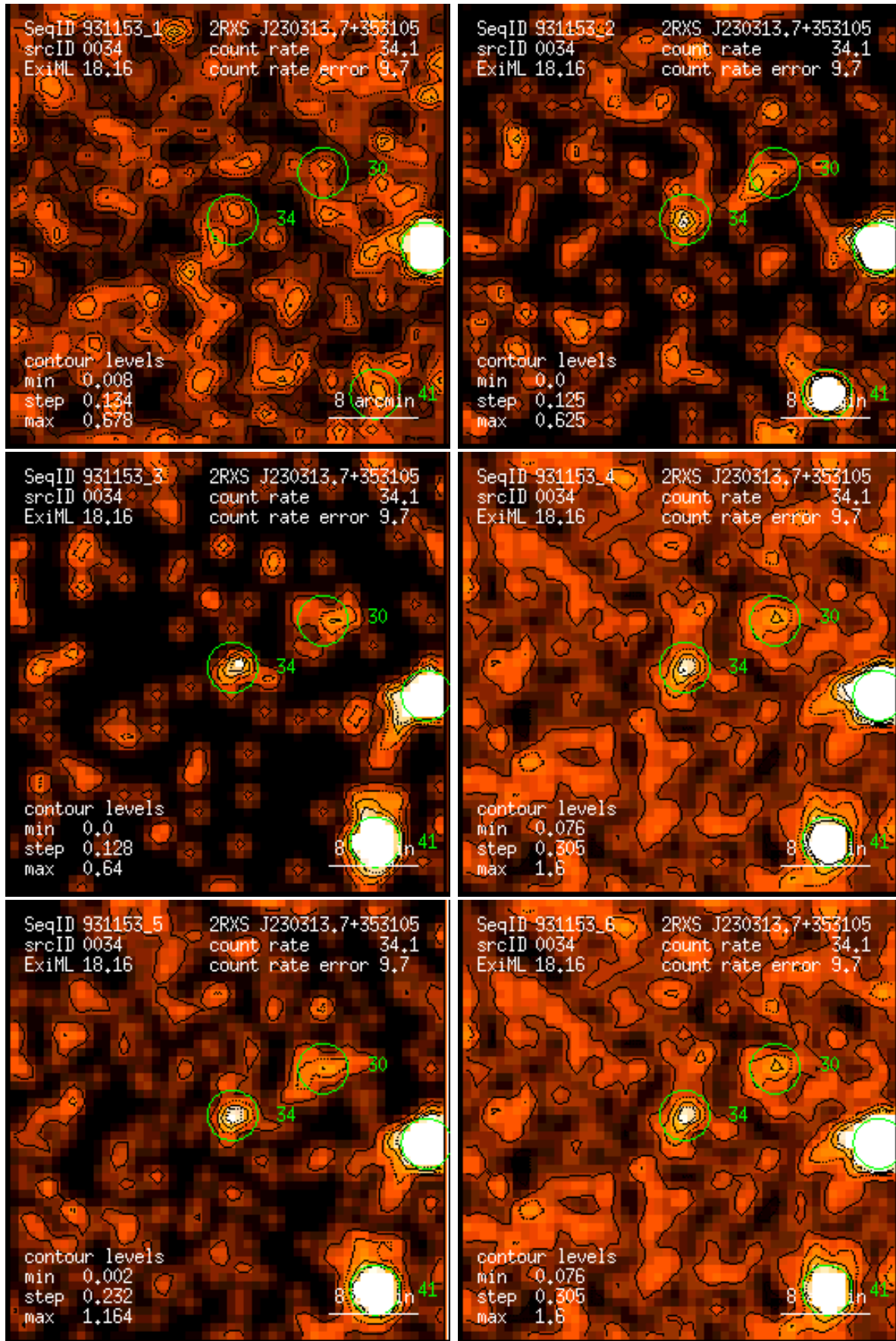
Figure 34: RASS 931153: detection 0034: band rate images, Gaussian filter: (1) PSPC channels 11 – 41, (2) 52 – 90, (3) 91 – 201, (4) 11 – 235, (5) 52 – 201, (6) 11 – 201. Broad band rates in counts/ks. Band rate contour levels in counts/ks/arcmin 2 .
