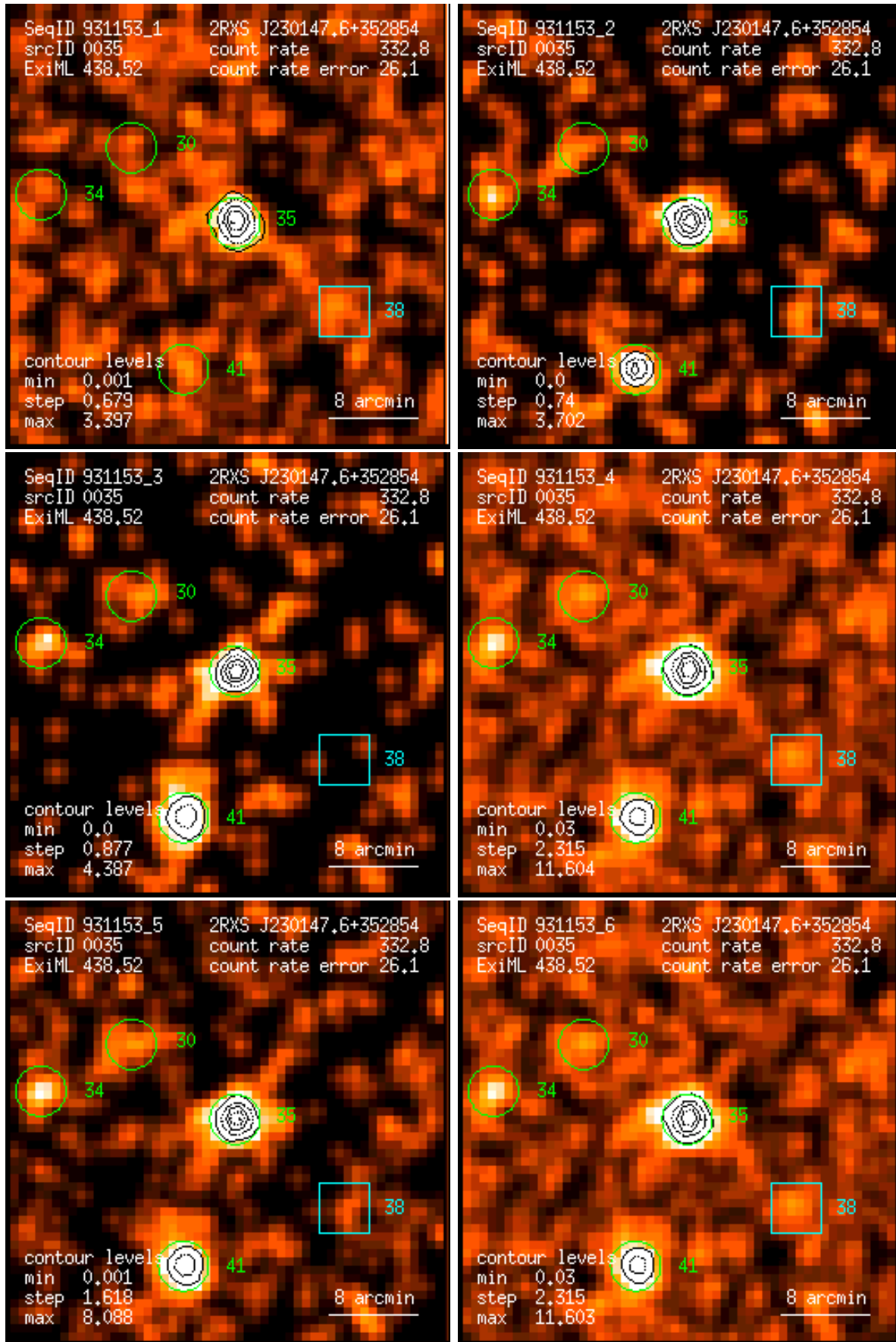
Figure 35: RASS 931153: detection 0035: band rate images, Gaussian filter: (1) PSPC channels 11 – 41, (2) 52 – 90, (3) 91 – 201, (4) 11 – 235, (5) 52 – 201, (6) 11 – 201. Broad band rates in counts/ks. Band rate contour levels in counts/ks/arcmin 2 .
