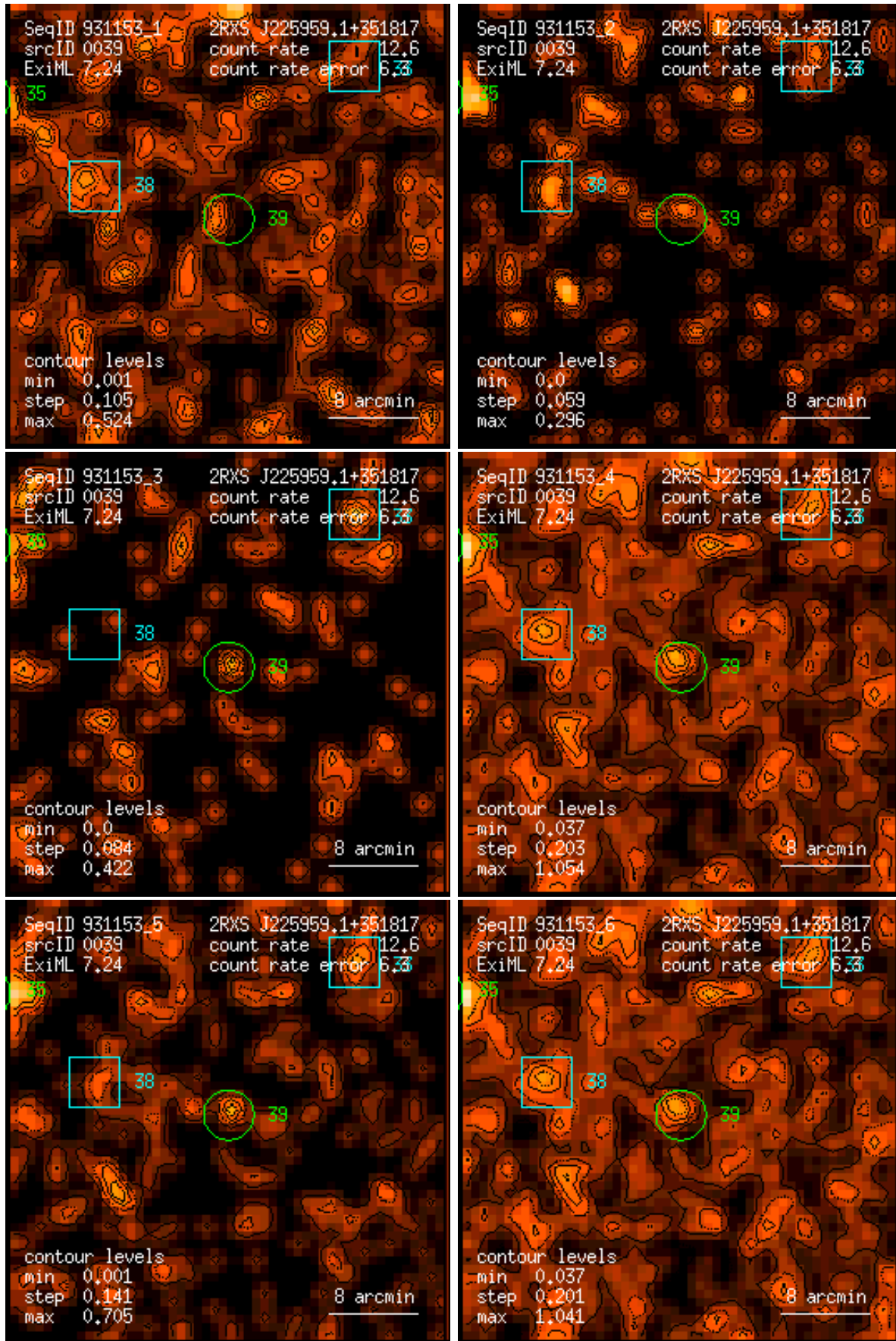
Figure 39: RASS 931153: detection 0039: band rate images, Gaussian filter: (1) PSPC channels 11 – 41, (2) 52 – 90, (3) 91 – 201, (4) 11 – 235, (5) 52 – 201, (6) 11 – 201. Broad band rates in counts/ks. Band rate contour levels in counts/ks/arcmin 2 .
