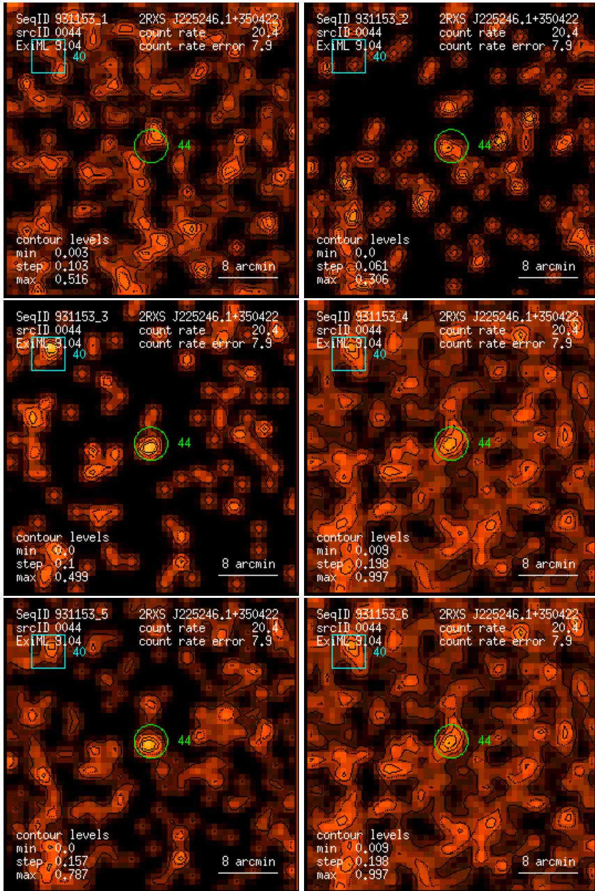
Figure 44: RASS 931153: detection 0044: band rate images, Gaussian filter: (1) PSPC channels 11 – 41, (2) 52 – 90, (3) 91 – 201, (4) 11 – 235, (5) 52 – 201, (6) 11 – 201. Broad band rates in counts/ks. Band rate contour levels in counts/ks/arcmin 2 .
