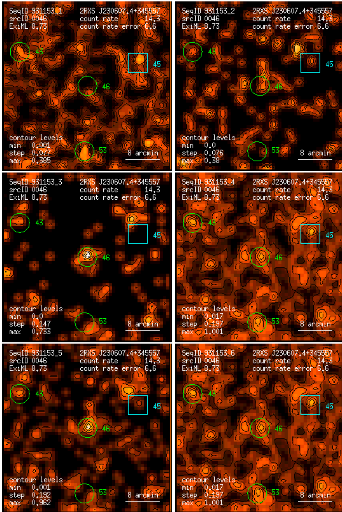
Figure 46: RASS 931153: detection 0046: band rate images, Gaussian filter: (1) PSPC channels 11 – 41, (2) 52 – 90, (3) 91 – 201, (4) 11 – 235, (5) 52 – 201, (6) 11 – 201. Broad band rates in counts/ks. Band rate contour levels in counts/ks/arcmin 2 .
