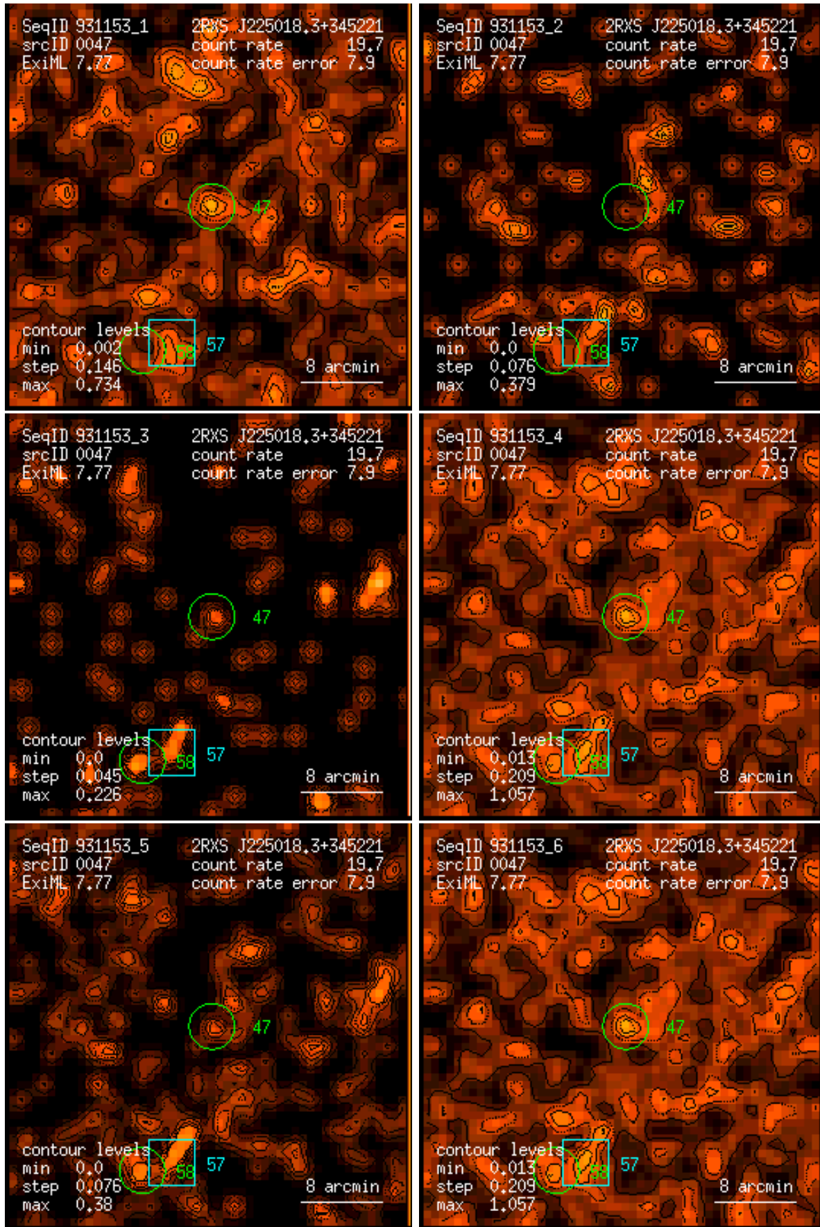
Figure 47: RASS 931153: detection 0047: band rate images, Gaussian filter: (1) PSPC channels 11 – 41, (2) 52 – 90, (3) 91 – 201, (4) 11 – 235, (5) 52 – 201, (6) 11 – 201. Broad band rates in counts/ks. Band rate contour levels in counts/ks/arcmin 2 .
