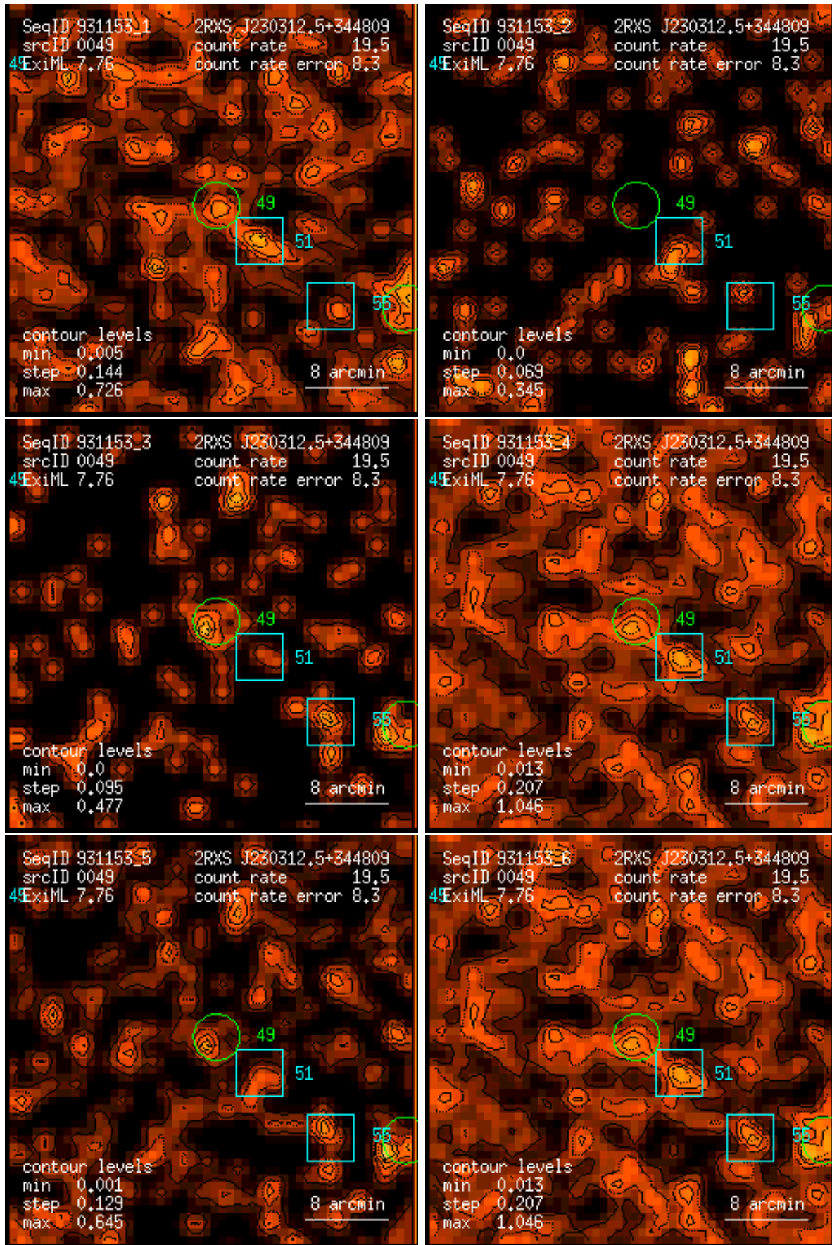
Figure 49: RASS 931153: detection 0049: band rate images, Gaussian filter: (1) PSPC channels 11 – 41, (2) 52 – 90, (3) 91 – 201, (4) 11 – 235, (5) 52 – 201, (6) 11 – 201. Broad band rates in counts/ks. Band rate contour levels in counts/ks/arcmin 2 .
