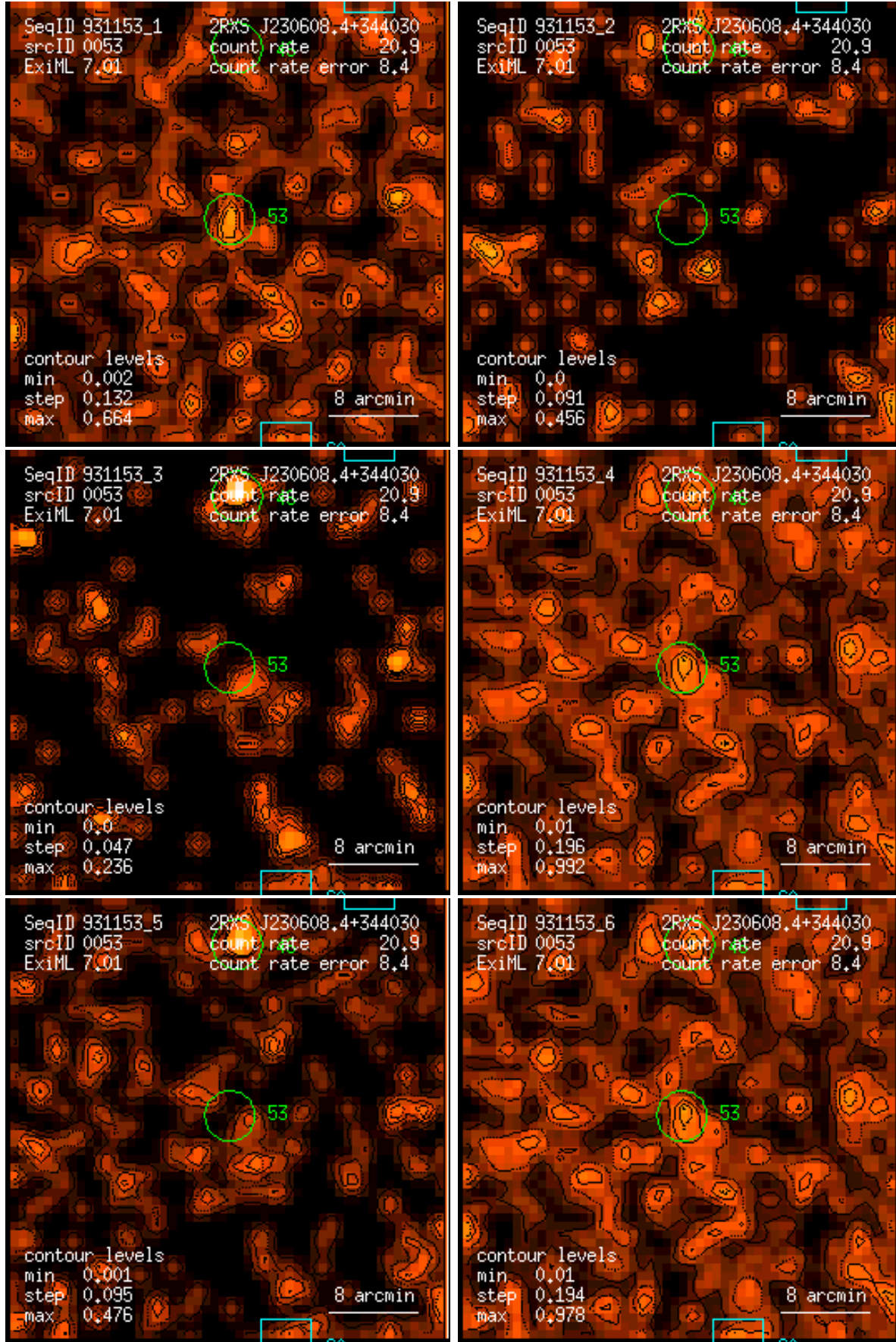
Figure 53: RASS 931153: detection 0053: band rate images, Gaussian filter: (1) PSPC channels 11 – 41, (2) 52 – 90, (3) 91 – 201, (4) 11 – 235, (5) 52 – 201, (6) 11 – 201. Broad band rates in counts/ks. Band rate contour levels in counts/ks/arcmin 2 .
