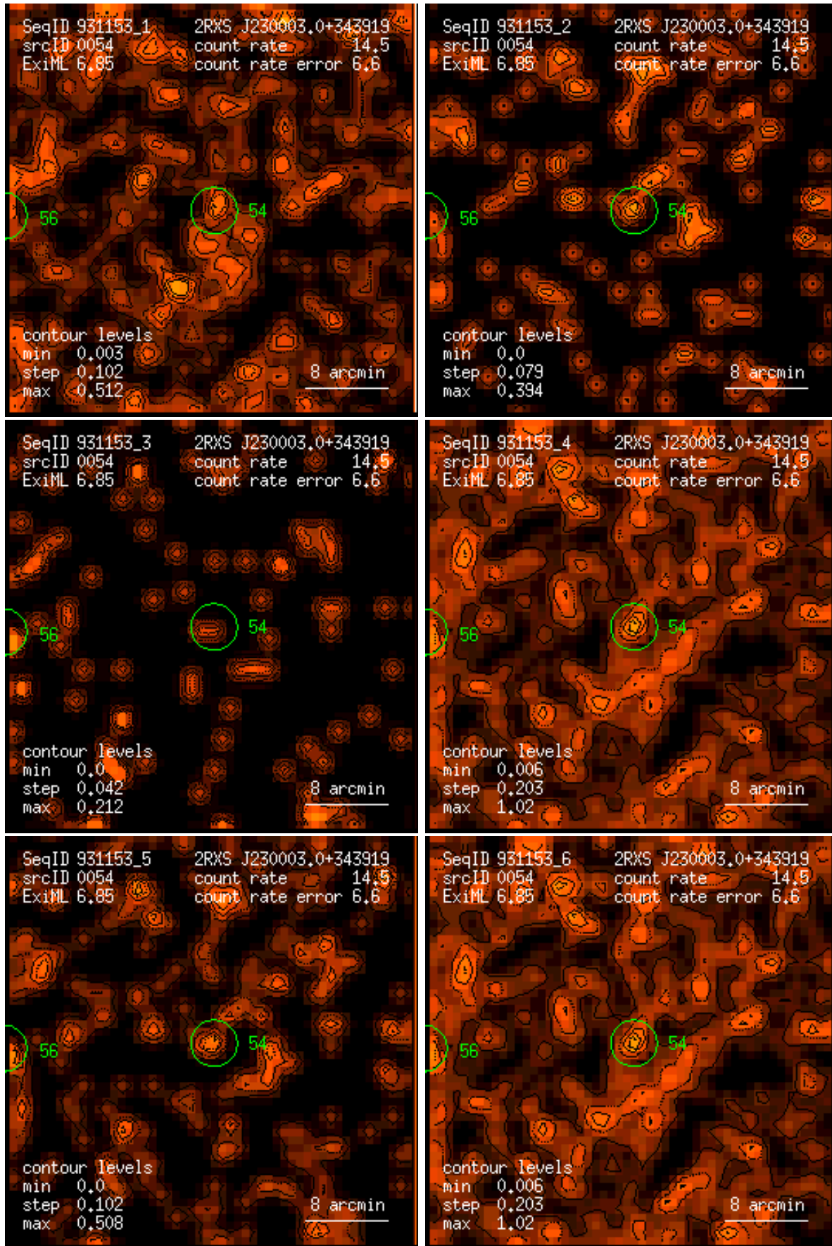
Figure 54: RASS 931153: detection 0054: band rate images, Gaussian filter: (1) PSPC channels 11 – 41, (2) 52 – 90, (3) 91 – 201, (4) 11 – 235, (5) 52 – 201, (6) 11 – 201. Broad band rates in counts/ks. Band rate contour levels in counts/ks/arcmin 2 .
