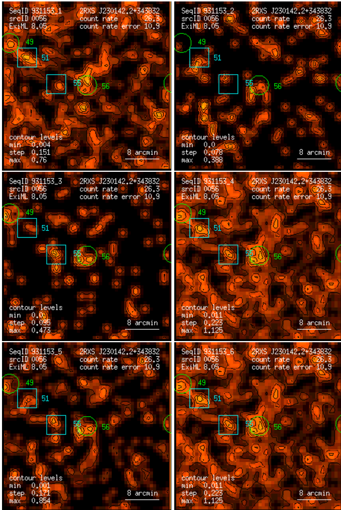
Figure 56: RASS 931153: detection 0056: band rate images, Gaussian filter: (1) PSPC channels 11 – 41, (2) 52 – 90, (3) 91 – 201, (4) 11 – 235, (5) 52 – 201, (6) 11 – 201. Broad band rates in counts/ks. Band rate contour levels in counts/ks/arcmin 2 .
