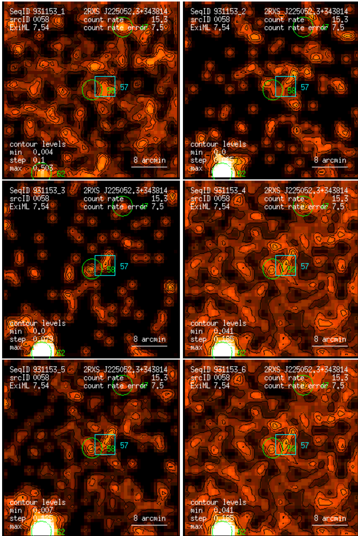
Figure 58: RASS 931153: detection 0058: band rate images, Gaussian filter: (1) PSPC channels 11 – 41, (2) 52 – 90, (3) 91 – 201, (4) 11 – 235, (5) 52 – 201, (6) 11 – 201. Broad band rates in counts/ks. Band rate contour levels in counts/ks/arcmin 2 .
