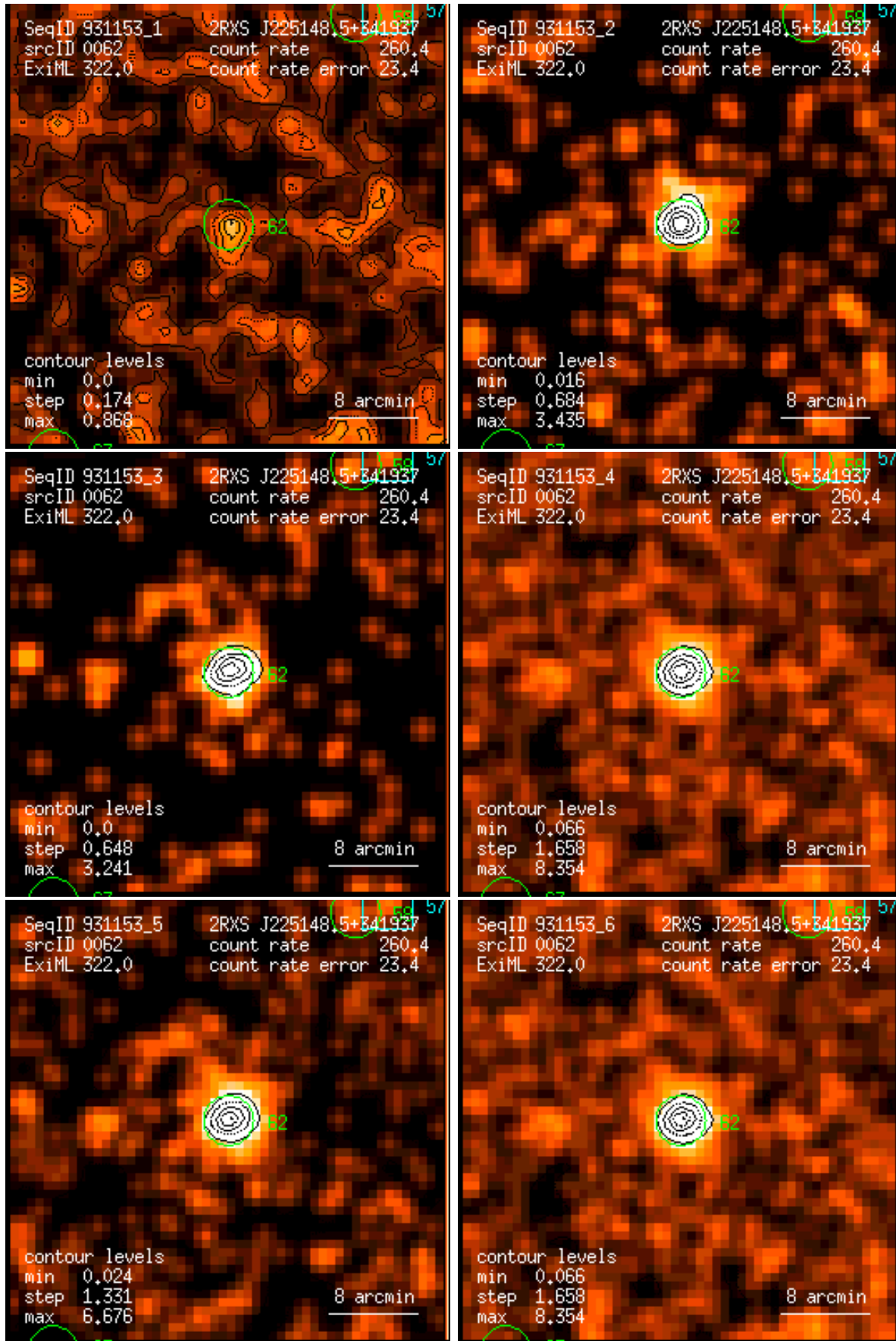
Figure 62: RASS 931153: detection 0062: band rate images, Gaussian filter: (1) PSPC channels 11 – 41, (2) 52 – 90, (3) 91 – 201, (4) 11 – 235, (5) 52 – 201, (6) 11 – 201. Broad band rates in counts/ks. Band rate contour levels in counts/ks/arcmin 2 .
