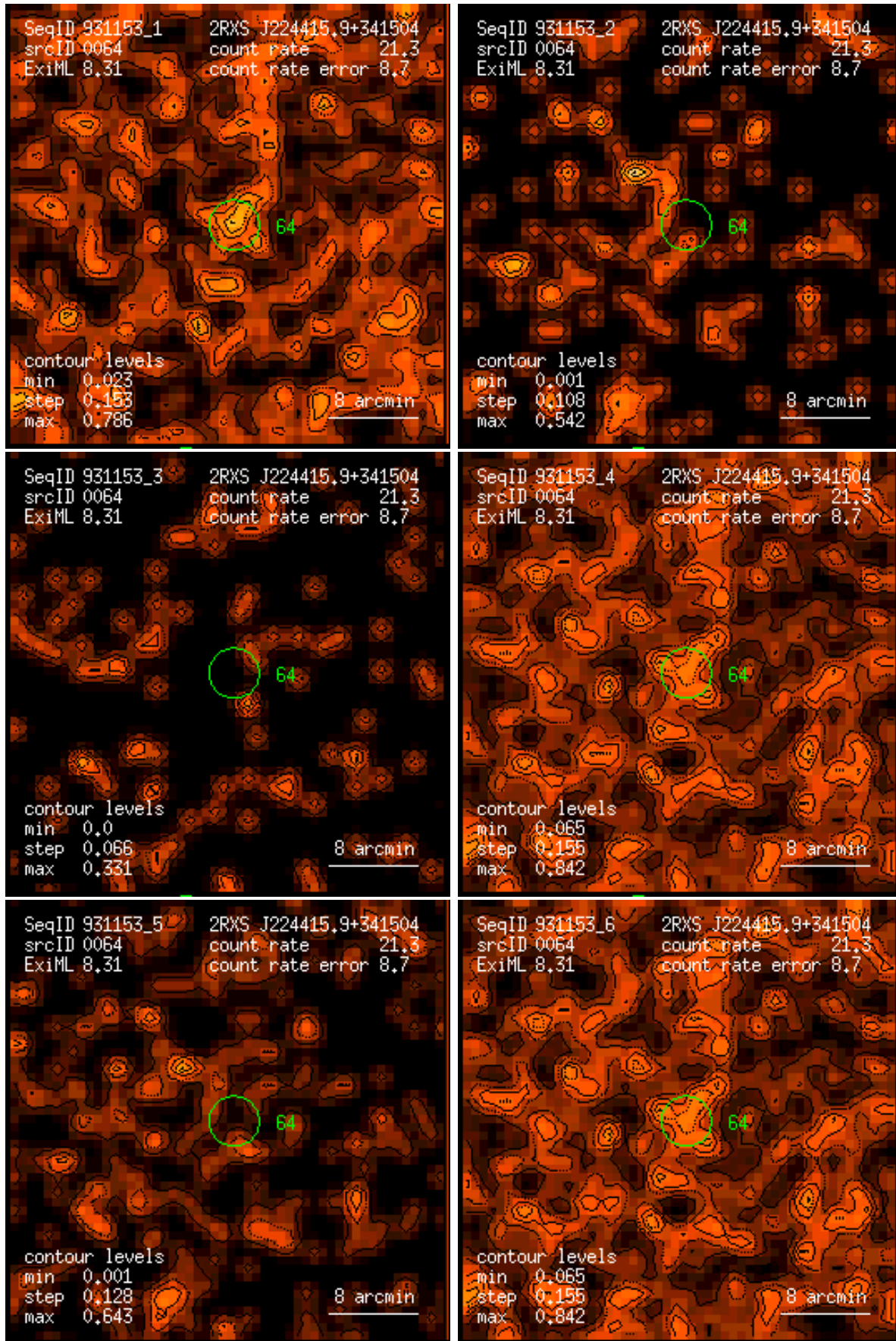
Figure 64: RASS 931153: detection 0064: band rate images, Gaussian filter: (1) PSPC channels 11 – 41, (2) 52 – 90, (3) 91 – 201, (4) 11 – 235, (5) 52 – 201, (6) 11 – 201. Broad band rates in counts/ks. Band rate contour levels in counts/ks/arcmin 2 .
