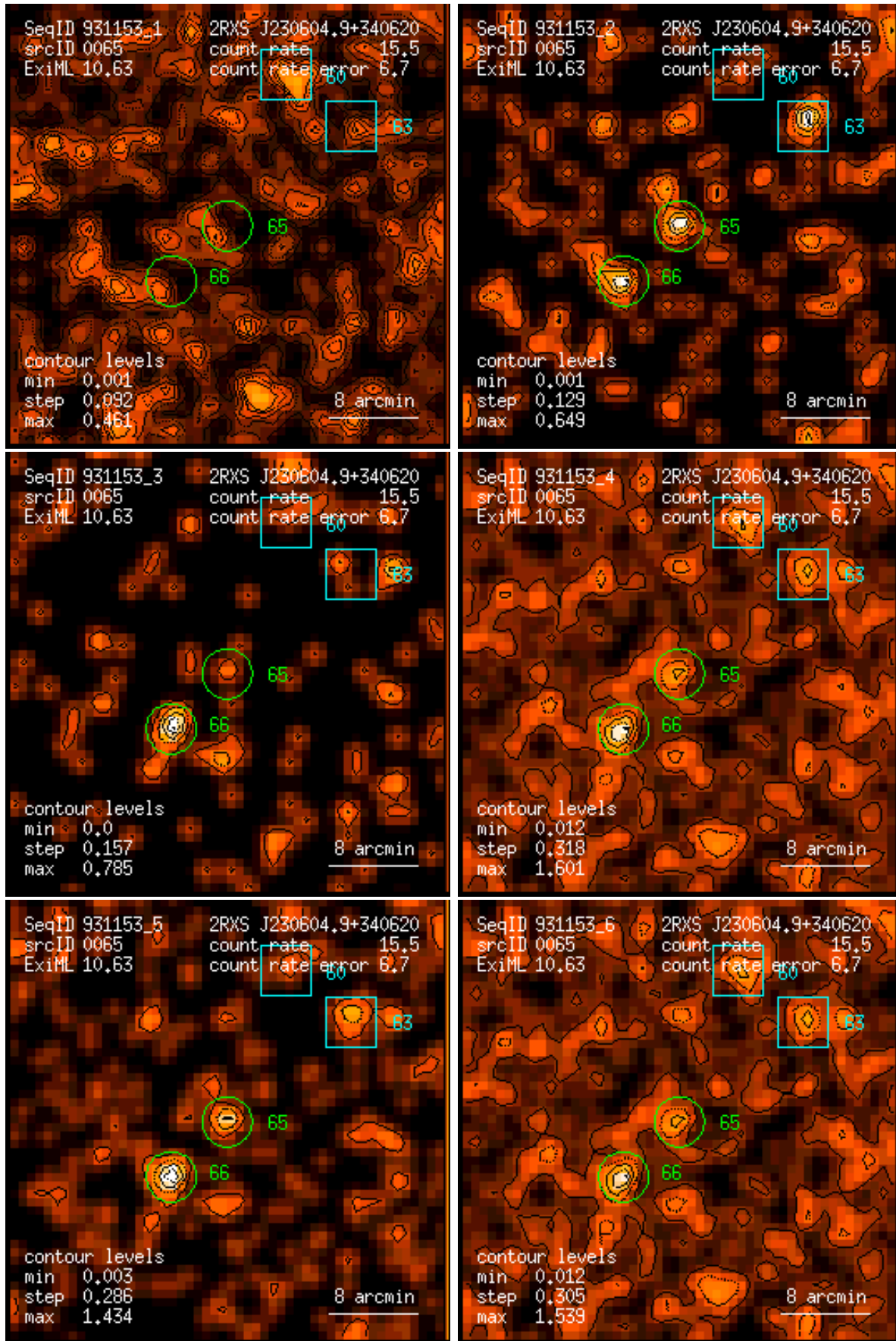
Figure 65: RASS 931153: detection 0065: band rate images, Gaussian filter: (1) PSPC channels 11 – 41, (2) 52 – 90, (3) 91 – 201, (4) 11 – 235, (5) 52 – 201, (6) 11 – 201. Broad band rates in counts/ks. Band rate contour levels in counts/ks/arcmin 2 .
