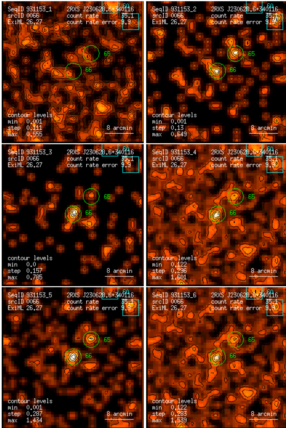
Figure 66: RASS 931153: detection 0066: band rate images, Gaussian filter: (1) PSPC channels 11 – 41, (2) 52 – 90, (3) 91 – 201, (4) 11 – 235, (5) 52 – 201, (6) 11 – 201. Broad band rates in counts/ks. Band rate contour levels in counts/ks/arcmin 2 .
