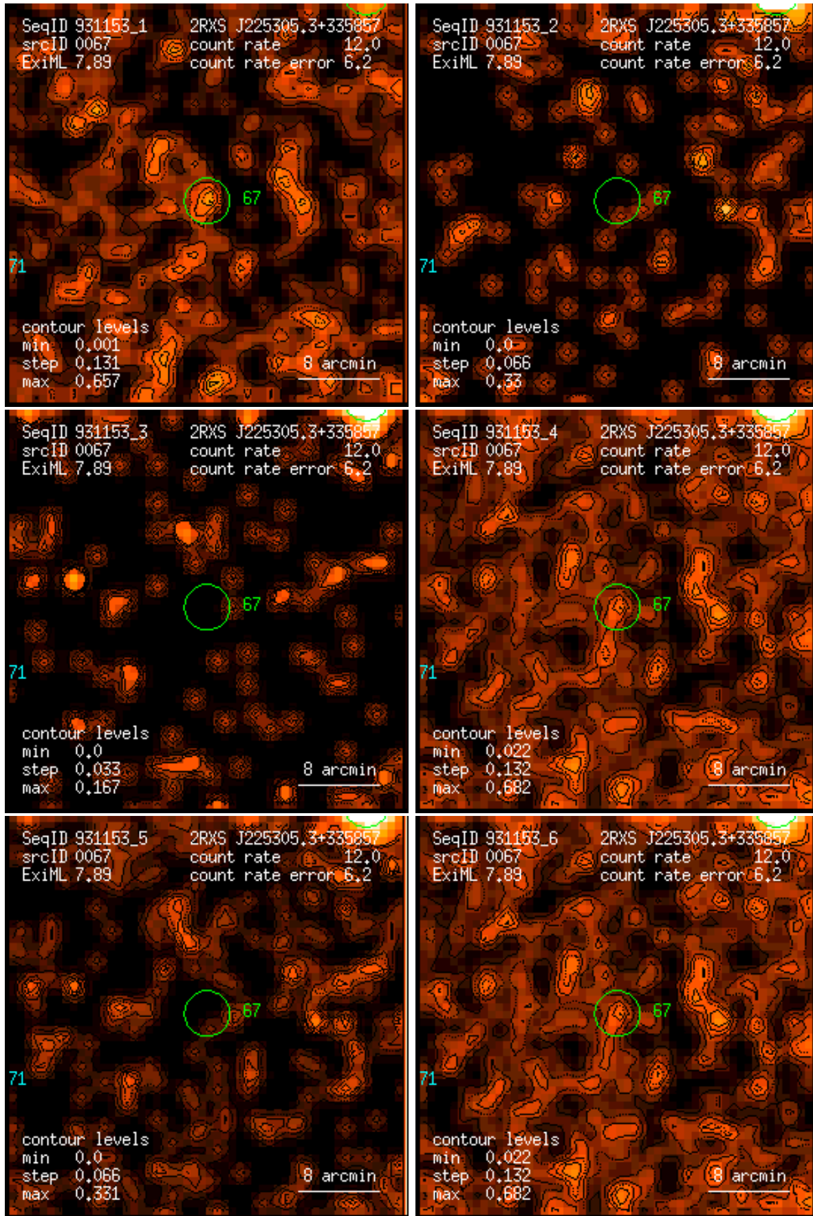
Figure 67: RASS 931153: detection 0067: band rate images, Gaussian filter: (1) PSPC channels 11 – 41, (2) 52 – 90, (3) 91 – 201, (4) 11 – 235, (5) 52 – 201, (6) 11 – 201. Broad band rates in counts/ks. Band rate contour levels in counts/ks/arcmin 2 .
