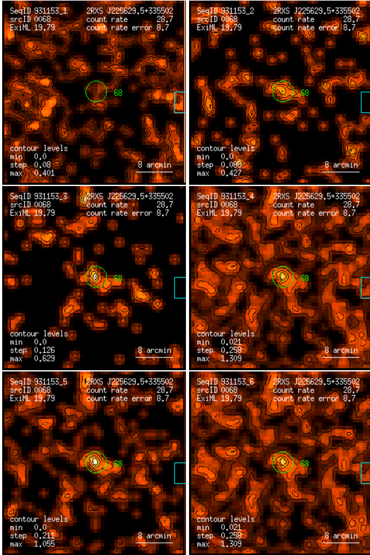
Figure 68: RASS 931153: detection 0068: band rate images, Gaussian filter: (1) PSPC channels 11 – 41, (2) 52 – 90, (3) 91 – 201, (4) 11 – 235, (5) 52 – 201, (6) 11 – 201. Broad band rates in counts/ks. Band rate contour levels in counts/ks/arcmin 2 .
