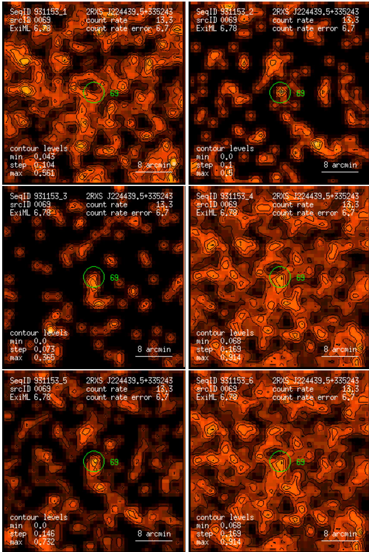
Figure 69: RASS 931153: detection 0069: band rate images, Gaussian filter: (1) PSPC channels 11 – 41, (2) 52 – 90, (3) 91 – 201, (4) 11 – 235, (5) 52 – 201, (6) 11 – 201. Broad band rates in counts/ks. Band rate contour levels in counts/ks/arcmin 2 .
