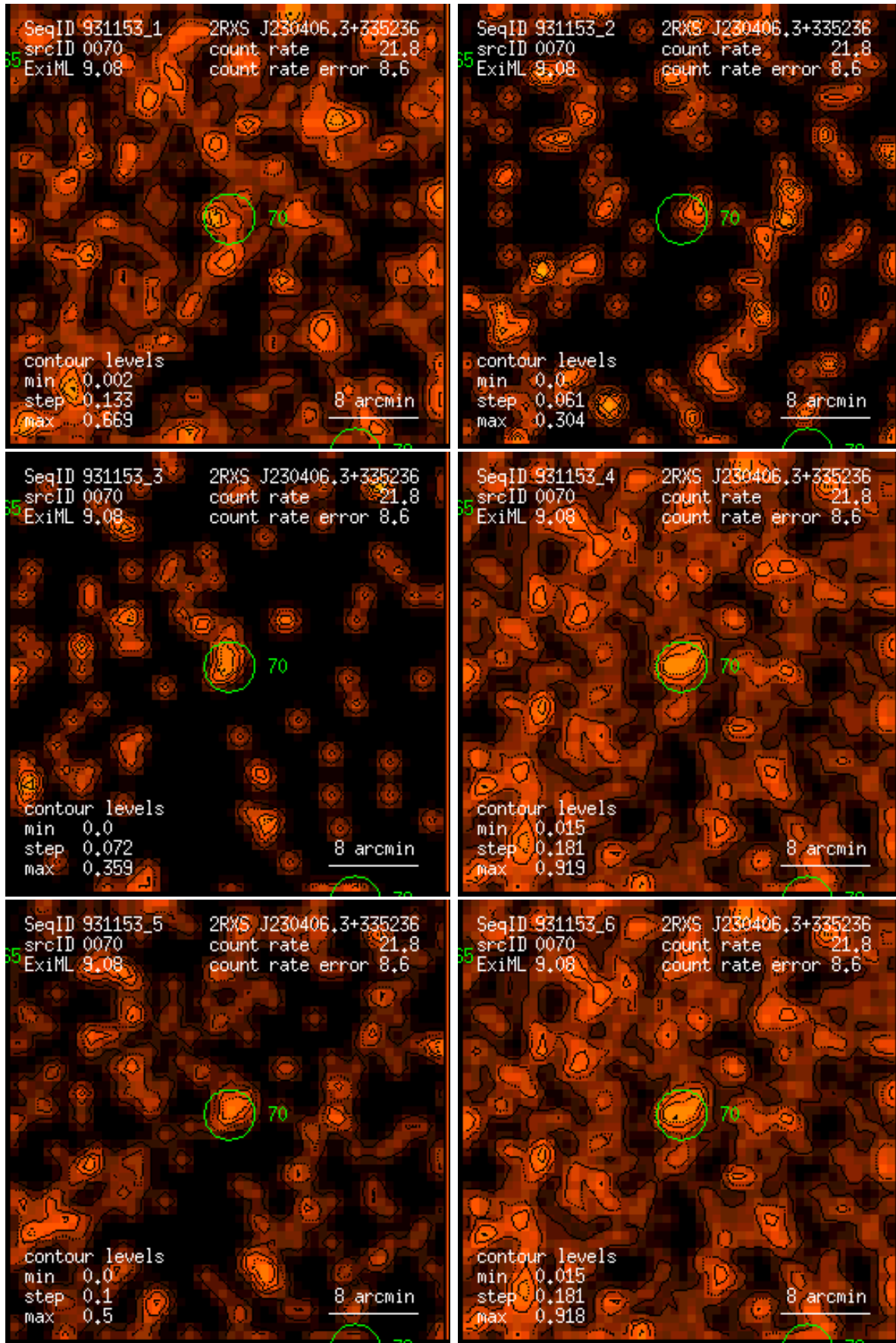
Figure 70: RASS 931153: detection 0070: band rate images, Gaussian filter: (1) PSPC channels 11 – 41, (2) 52 – 90, (3) 91 – 201, (4) 11 – 235, (5) 52 – 201, (6) 11 – 201. Broad band rates in counts/ks. Band rate contour levels in counts/ks/arcmin 2 .
