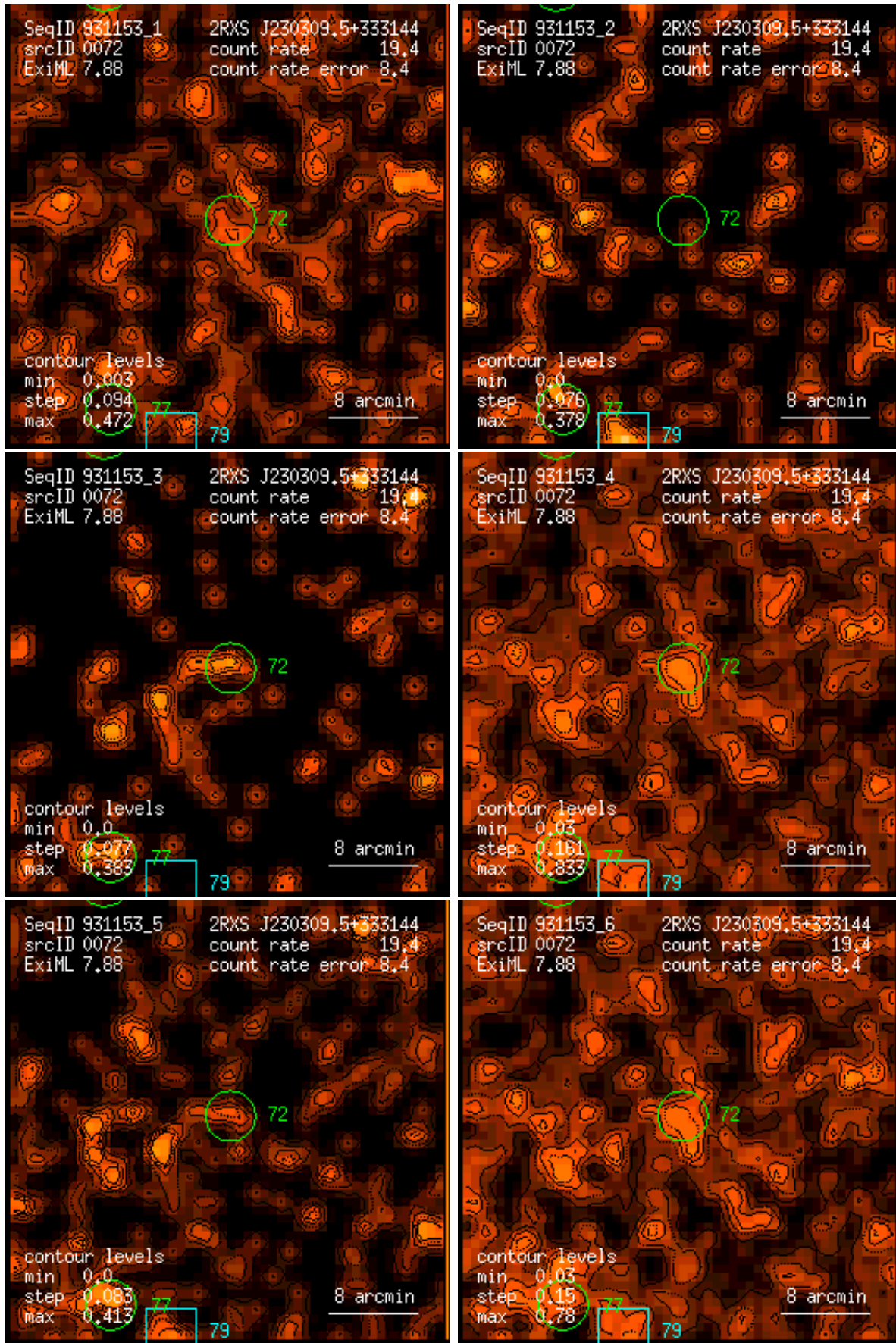
Figure 72: RASS 931153: detection 0072: band rate images, Gaussian filter: (1) PSPC channels 11 – 41, (2) 52 – 90, (3) 91 – 201, (4) 11 – 235, (5) 52 – 201, (6) 11 – 201. Broad band rates in counts/ks. Band rate contour levels in counts/ks/arcmin 2 .
