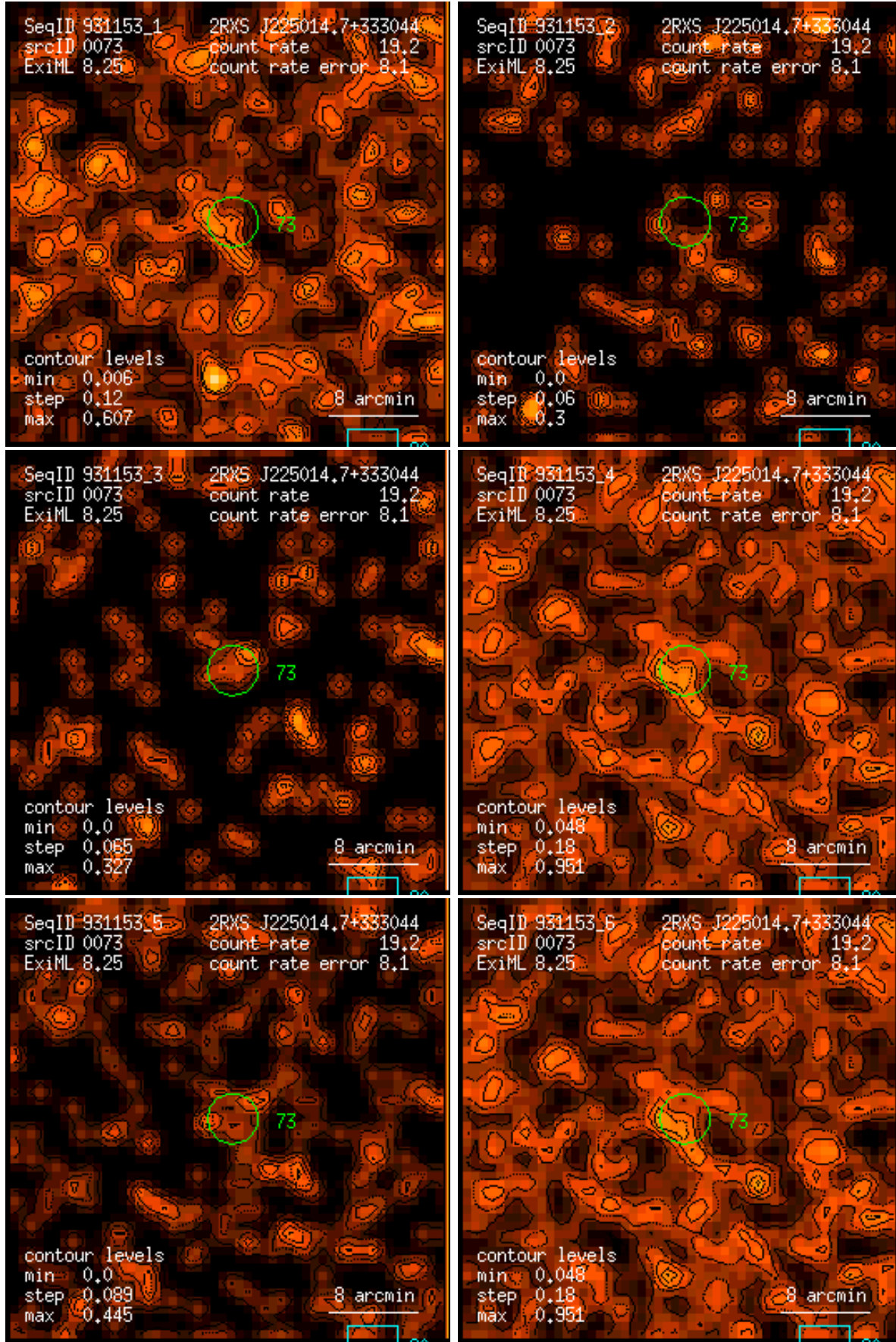
Figure 73: RASS 931153: detection 0073: band rate images, Gaussian filter: (1) PSPC channels 11 – 41, (2) 52 – 90, (3) 91 – 201, (4) 11 – 235, (5) 52 – 201, (6) 11 – 201. Broad band rates in counts/ks. Band rate contour levels in counts/ks/arcmin 2 .
