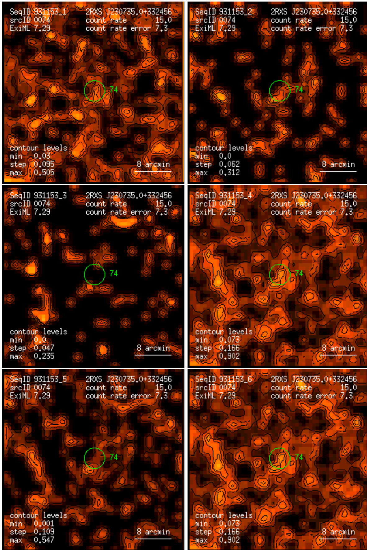
Figure 74: RASS 931153: detection 0074: band rate images, Gaussian filter: (1) PSPC channels 11 – 41, (2) 52 – 90, (3) 91 – 201, (4) 11 – 235, (5) 52 – 201, (6) 11 – 201. Broad band rates in counts/ks. Band rate contour levels in counts/ks/arcmin 2 .
