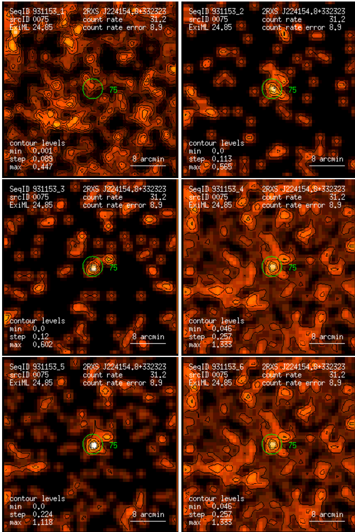
Figure 75: RASS 931153: detection 0075: band rate images, Gaussian filter: (1) PSPC channels 11 – 41, (2) 52 – 90, (3) 91 – 201, (4) 11 – 235, (5) 52 – 201, (6) 11 – 201. Broad band rates in counts/ks. Band rate contour levels in counts/ks/arcmin 2 .
