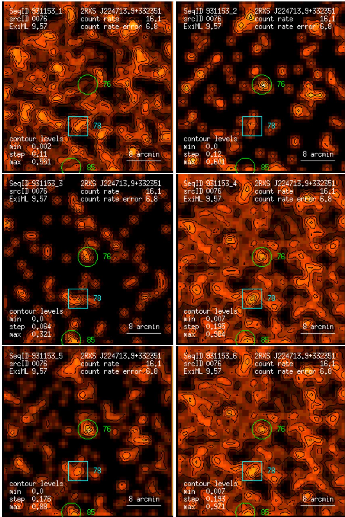
Figure 76: RASS 931153: detection 0076: band rate images, Gaussian filter: (1) PSPC channels 11 – 41, (2) 52 – 90, (3) 91 – 201, (4) 11 – 235, (5) 52 – 201, (6) 11 – 201. Broad band rates in counts/ks. Band rate contour levels in counts/ks/arcmin 2 .
