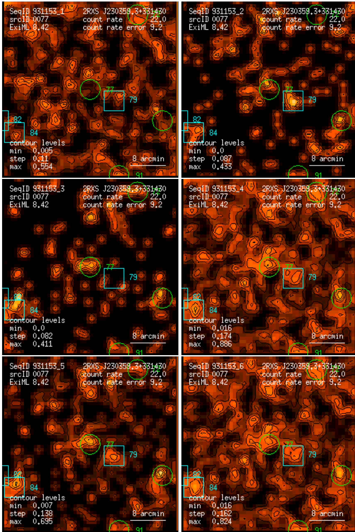
Figure 77: RASS 931153: detection 0077: band rate images, Gaussian filter: (1) PSPC channels 11 – 41, (2) 52 – 90, (3) 91 – 201, (4) 11 – 235, (5) 52 – 201, (6) 11 – 201. Broad band rates in counts/ks. Band rate contour levels in counts/ks/arcmin 2 .
