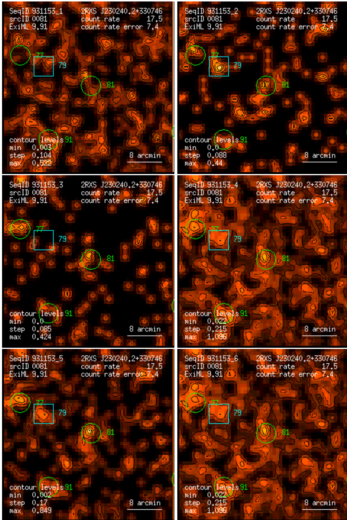
Figure 81: RASS 931153: detection 0081: band rate images, Gaussian filter: (1) PSPC channels 11 – 41, (2) 52 – 90, (3) 91 – 201, (4) 11 – 235, (5) 52 – 201, (6) 11 – 201. Broad band rates in counts/ks. Band rate contour levels in counts/ks/arcmin 2 .
