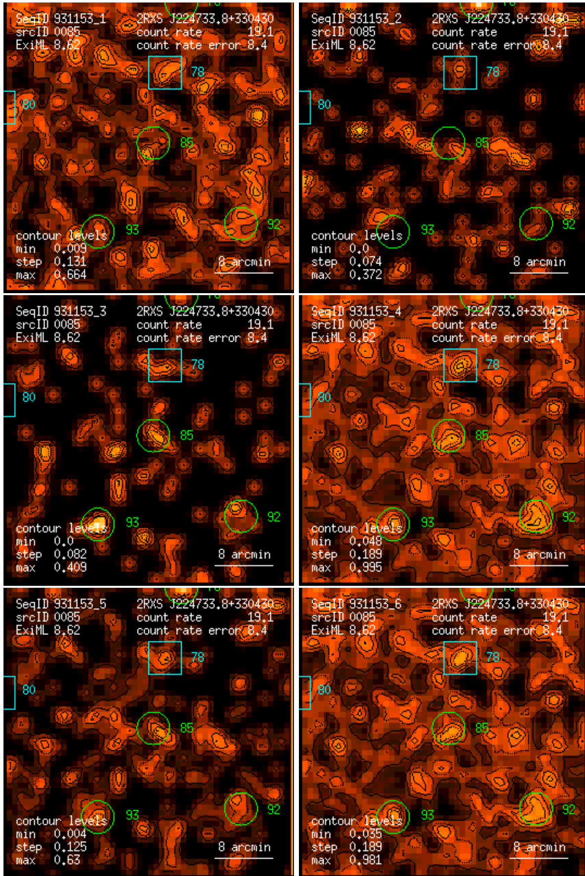
Figure 85: RASS 931153: detection 0085: band rate images, Gaussian filter: (1) PSPC channels 11 – 41, (2) 52 – 90, (3) 91 – 201, (4) 11 – 235, (5) 52 – 201, (6) 11 – 201. Broad band rates in counts/ks. Band rate contour levels in counts/ks/arcmin 2 .
