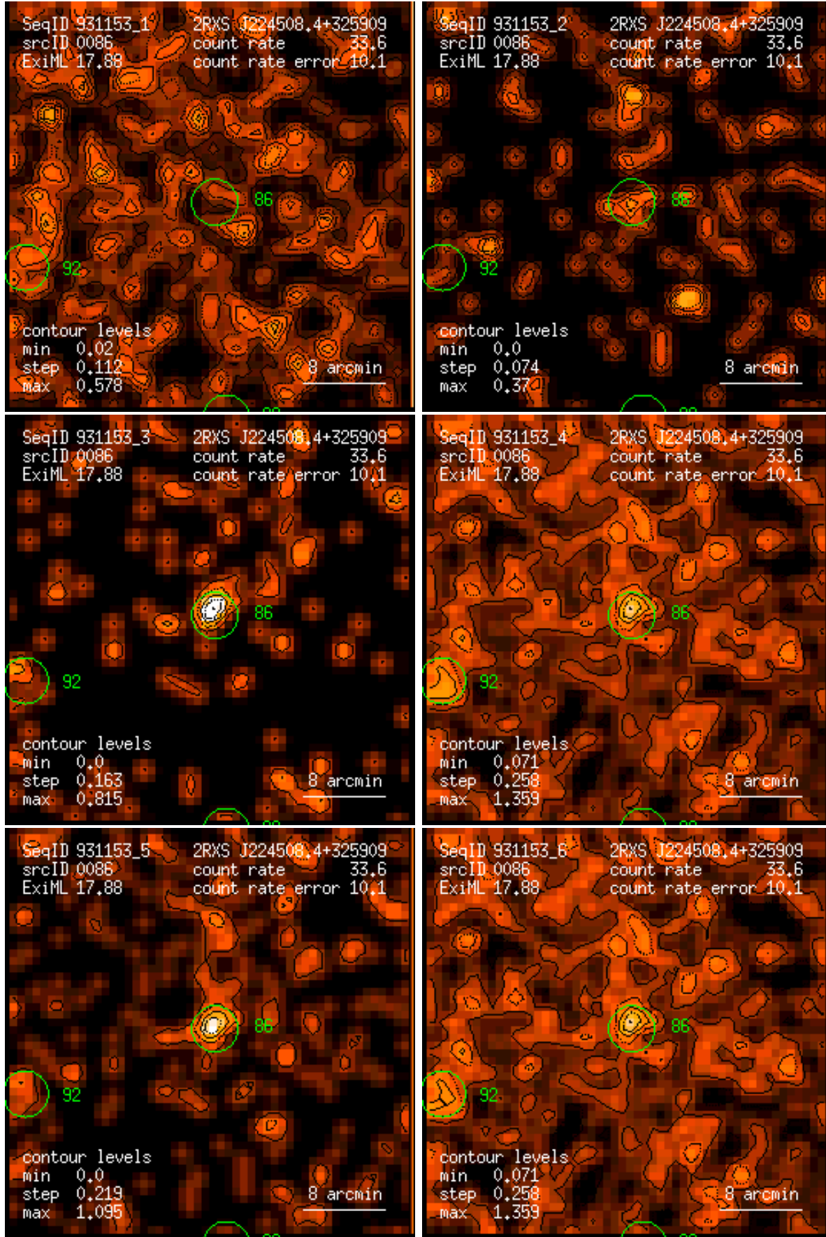
Figure 86: RASS 931153: detection 0086: band rate images, Gaussian filter: (1) PSPC channels 11 – 41, (2) 52 – 90, (3) 91 – 201, (4) 11 – 235, (5) 52 – 201, (6) 11 – 201. Broad band rates in counts/ks. Band rate contour levels in counts/ks/arcmin 2 .
