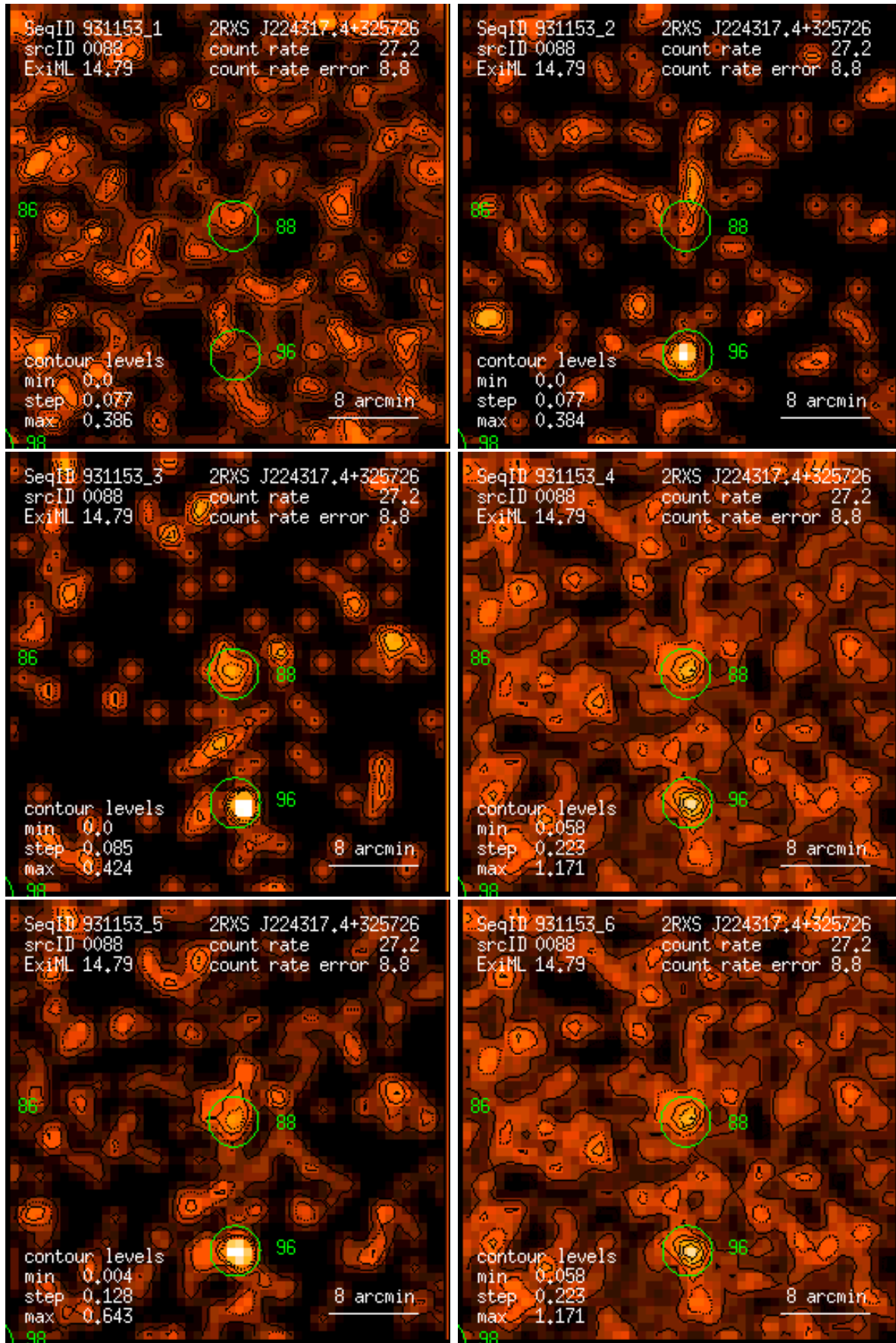
Figure 88: RASS 931153: detection 0088: band rate images, Gaussian filter: (1) PSPC channels 11 – 41, (2) 52 – 90, (3) 91 – 201, (4) 11 – 235, (5) 52 – 201, (6) 11 – 201. Broad band rates in counts/ks. Band rate contour levels in counts/ks/arcmin 2 .
