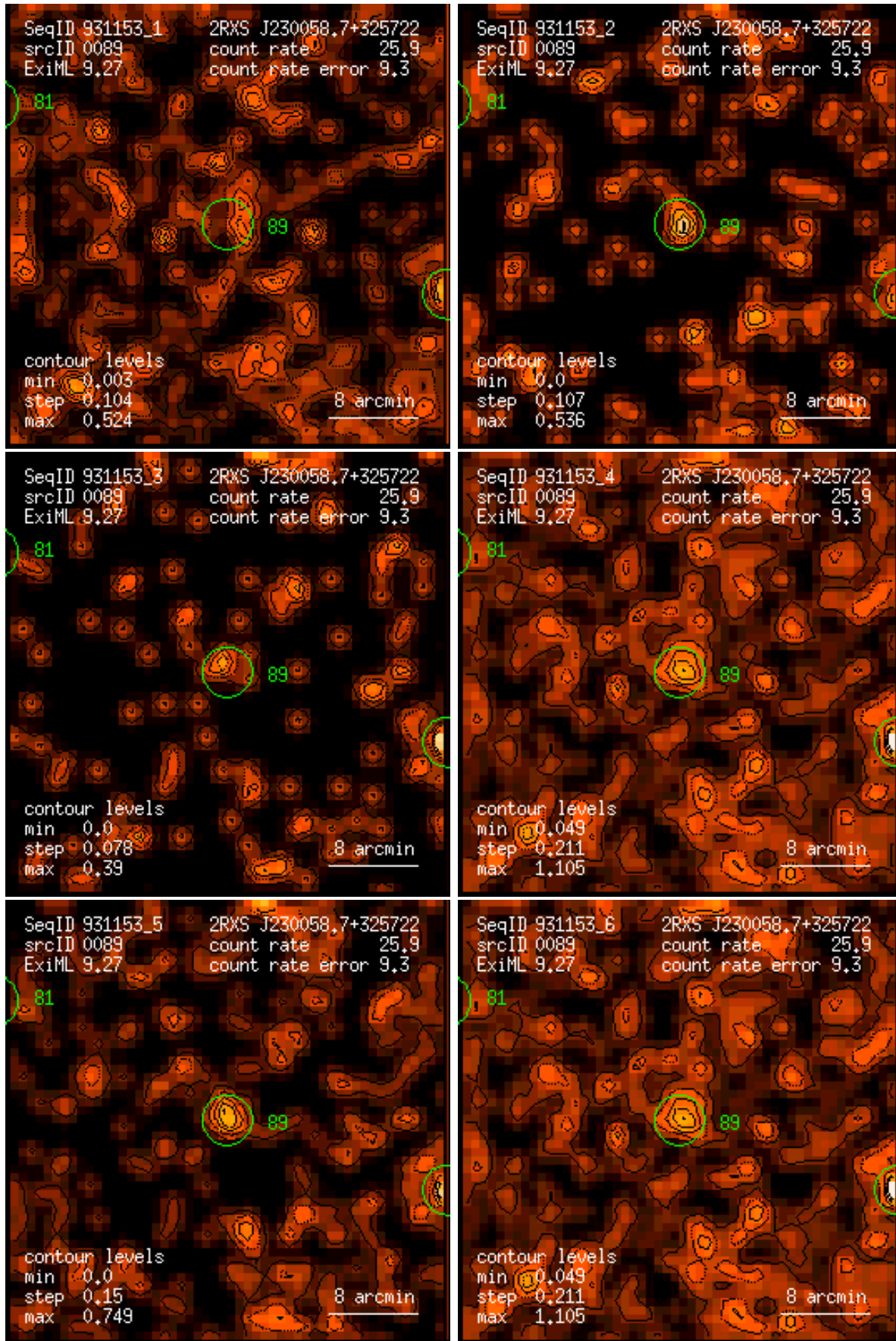
Figure 89: RASS 931153: detection 0089: band rate images, Gaussian filter: (1) PSPC channels 11 – 41, (2) 52 – 90, (3) 91 – 201, (4) 11 – 235, (5) 52 – 201, (6) 11 – 201. Broad band rates in counts/ks. Band rate contour levels in counts/ks/arcmin 2 .
