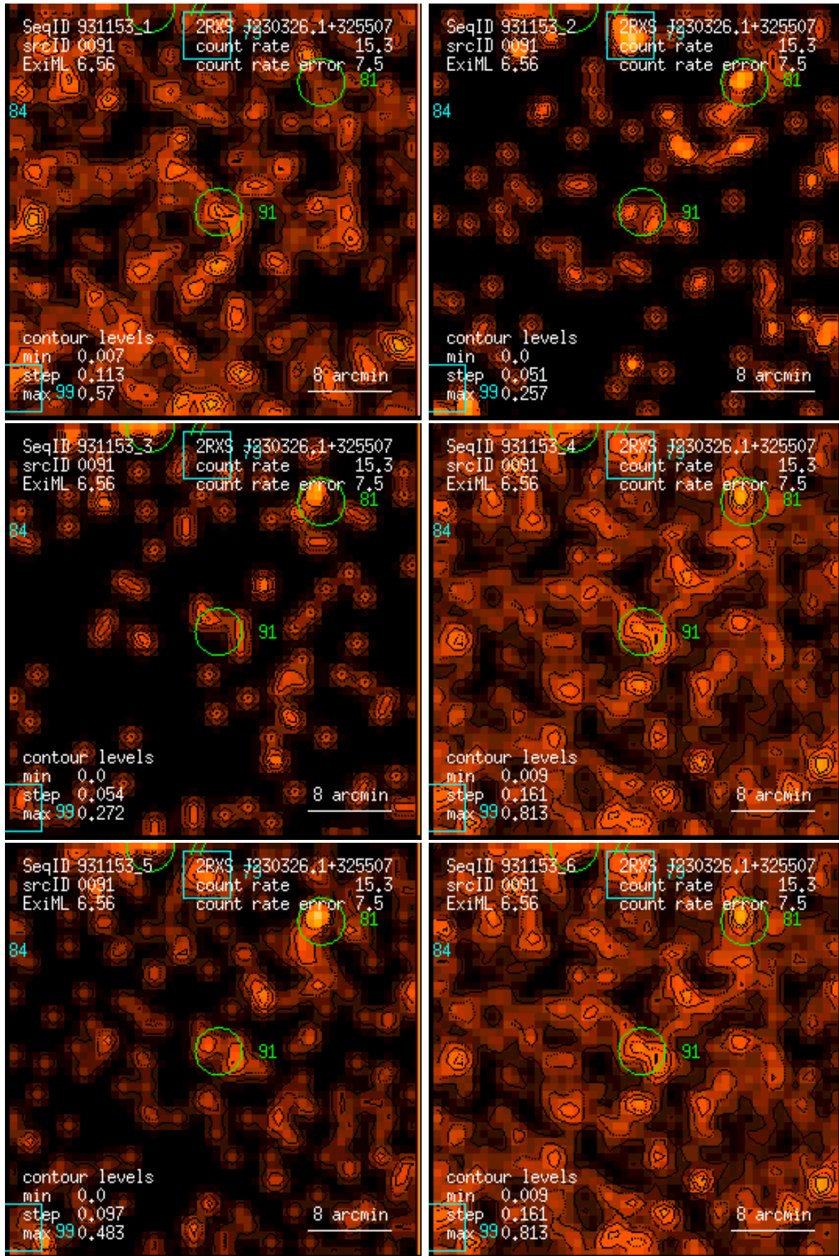
Figure 91: RASS 931153: detection 0091: band rate images, Gaussian filter: (1) PSPC channels 11 – 41, (2) 52 – 90, (3) 91 – 201, (4) 11 – 235, (5) 52 – 201, (6) 11 – 201. Broad band rates in counts/ks. Band rate contour levels in counts/ks/arcmin 2 .
