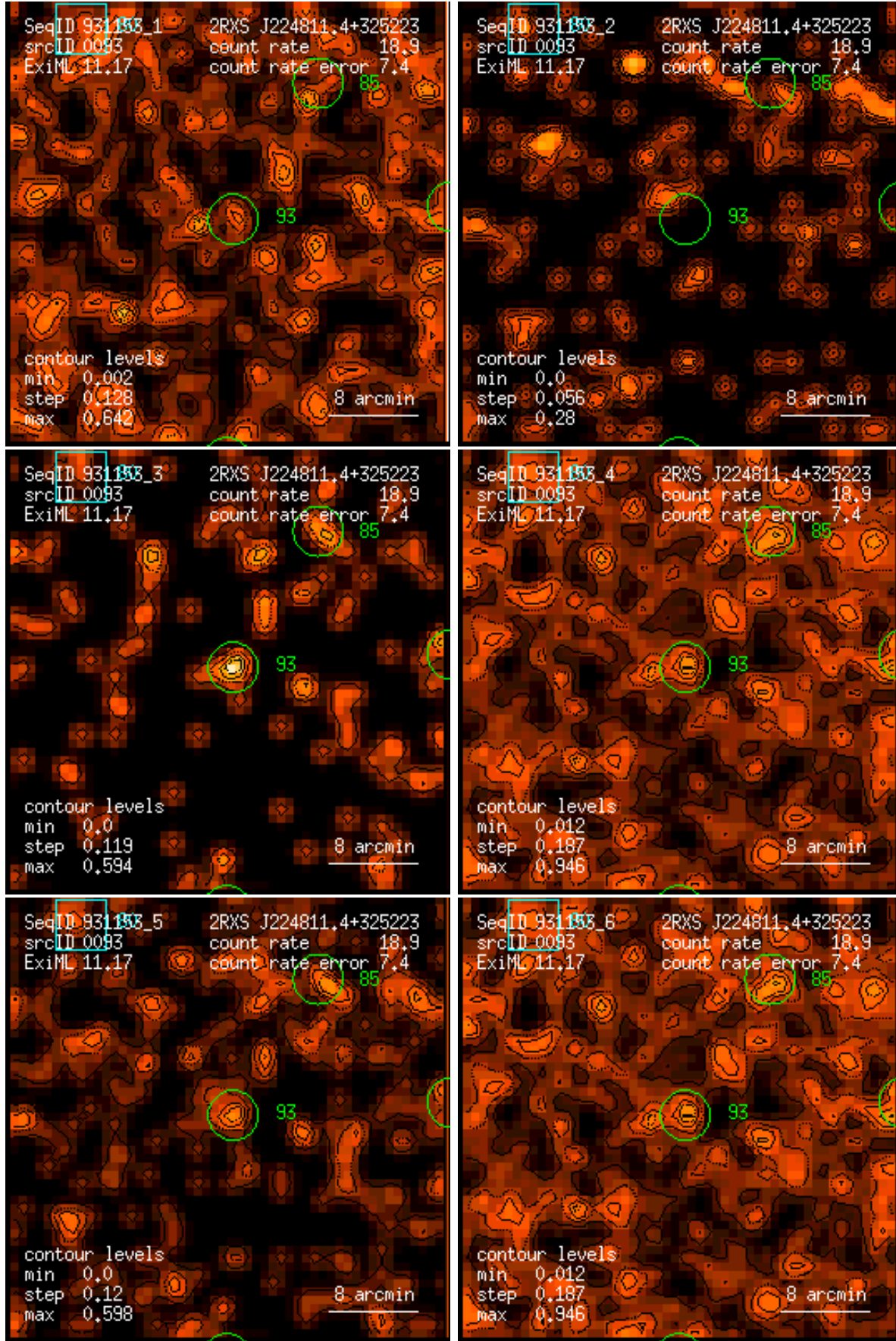
Figure 93: RASS 931153: detection 0093: band rate images, Gaussian filter: (1) PSPC channels 11 – 41, (2) 52 – 90, (3) 91 – 201, (4) 11 – 235, (5) 52 – 201, (6) 11 – 201. Broad band rates in counts/ks. Band rate contour levels in counts/ks/arcmin 2 .
