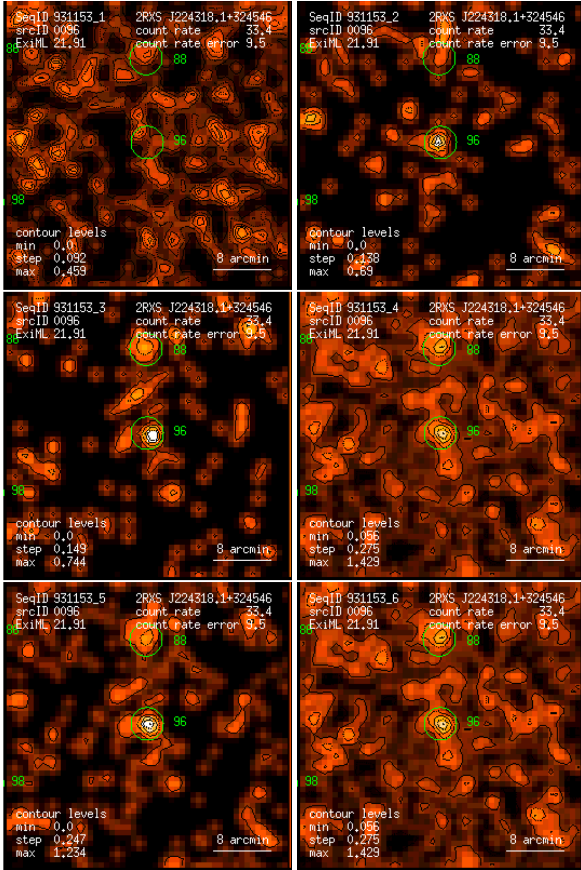
Figure 96: RASS 931153: detection 0096: band rate images, Gaussian filter: (1) PSPC channels 11 – 41, (2) 52 – 90, (3) 91 – 201, (4) 11 – 235, (5) 52 – 201, (6) 11 – 201. Broad band rates in counts/ks. Band rate contour levels in counts/ks/arcmin 2 .
